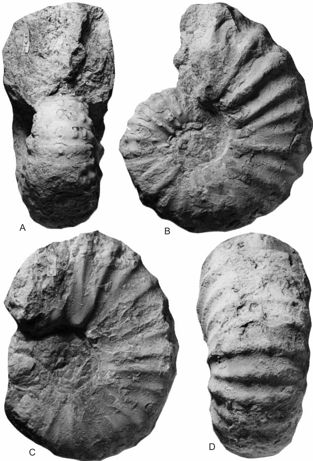
Text-fig. 18. A, B— Romaniceras ( Yubariceras ) ornatissimum (Stoliczka, 1865), FSIT MC15, from the Calcaires de Montplaisir (Saint-Louis syncline). C, D— Romaniceras ( Romaniceras ) mexicanum Jones, 1938, FSIT CT6, from Les Capitaines. All figures are \times 1
