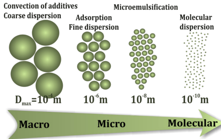
Fig. 1. Mechanism of emulsions' formation with different degrees of dispersion (from the turbulent dispersion via turbulent diffusion to molecular dispersion)
