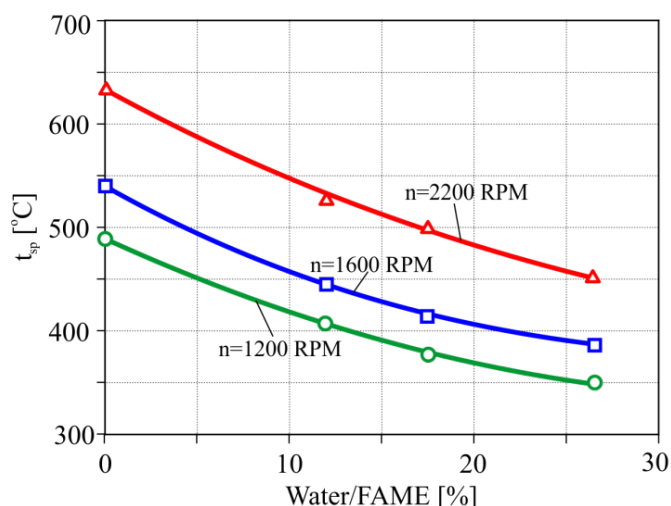
Fig. 14. Effect of water content of the emulsion FAME – water on the exhaust gases temperature
