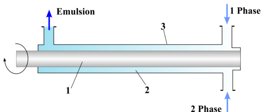
Fig. 2. Schematic of the helical mixer: Phase 1 – diesel oil or FAME fuel; Phase 2 – water with the possible surfactant content; 1 – rotor, 2 – the fuel-water emulsion, 3 – cylinder
