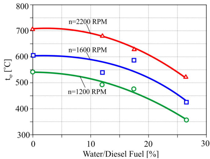
Fig. 13. Effect of water content of the fuel oil – water emulsion on the exhaust gases temperature
