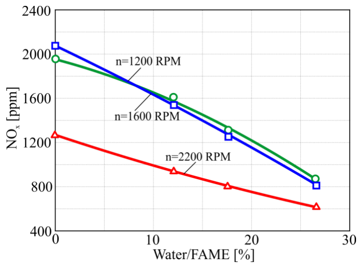
Fig. 8. Effect of water content of the FAME fuel – water emulsion on the emission of \text{NO}_x
