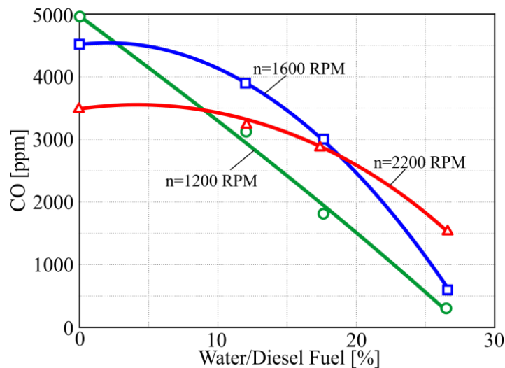
Fig. 5. Effect of water content of the fuel oil – water emulsion on the emission of carbon monoxide CO
