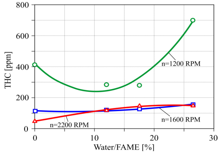
Fig. 4. Effect of water content of the FAME fuel – water emulsion on the emission of unburned hydrocarbons THC
