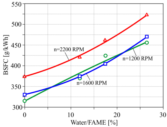
Fig. 12. Effect of water content of the FAME fuel – water emulsion on specific fuel consumption – BSFC
