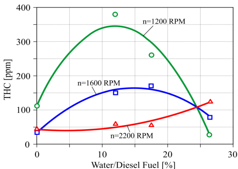
Fig. 3. Effect of water content of the fuel oil-water emulsion on the emission of unburned hydrocarbons THC
