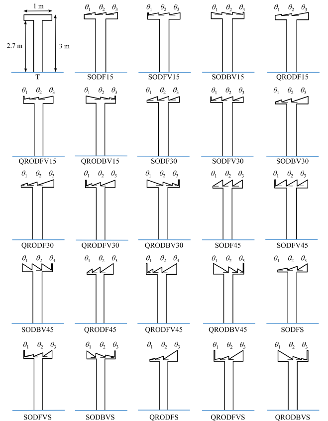
Fig. 1. The various designed noise barriers.
