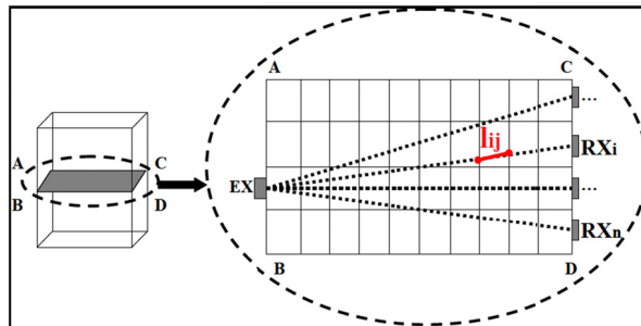
Fig. 8. Graphic display of the tomography ( l_{ij} is the wave length i in the cell j ) (Boviar, 2015)
