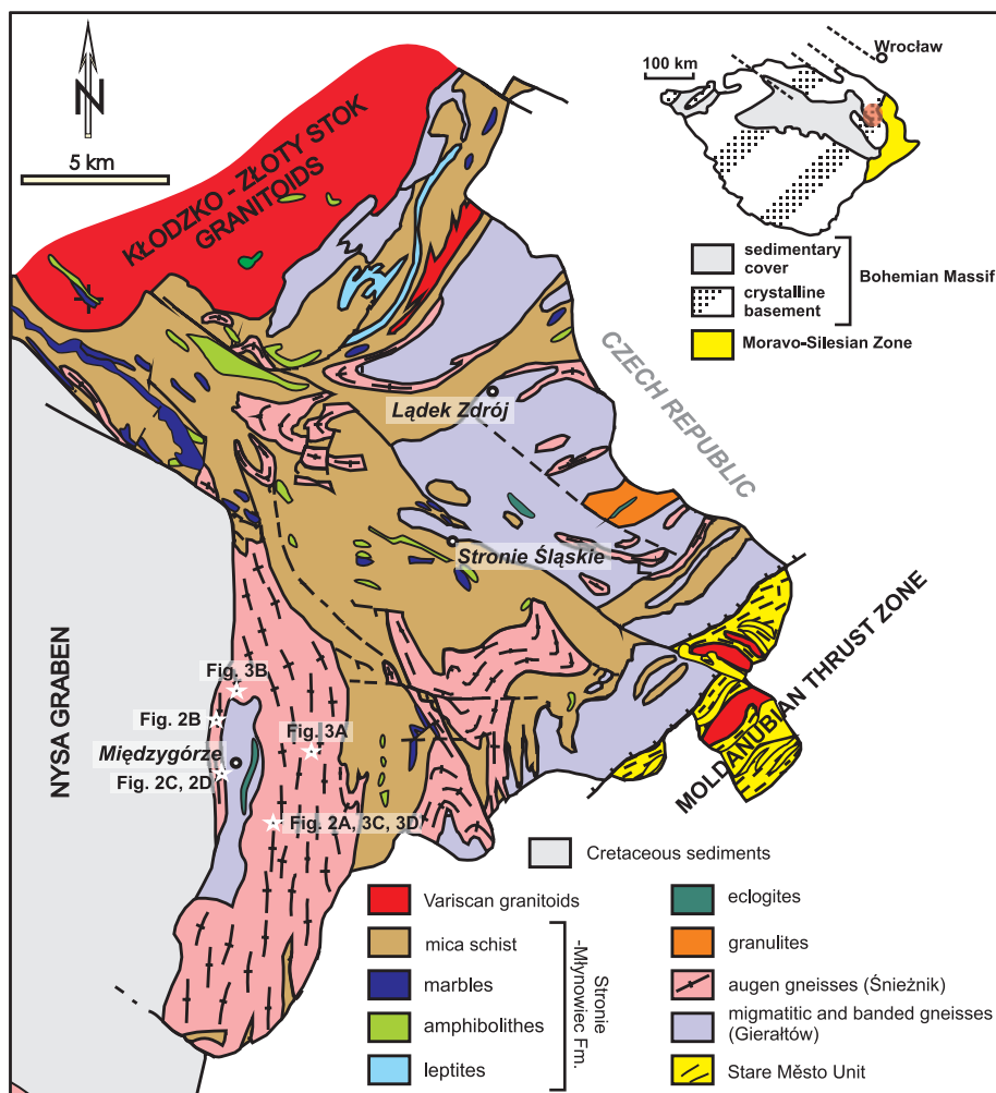
Fig. 1. Geological map of the eastern part of the Orlica-Śnieżnik Dome (modified after Don, 2001).
