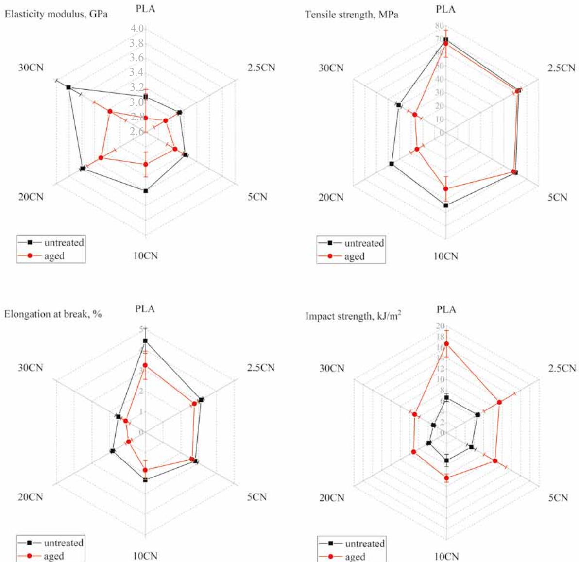
Fig. 2. Mechanical properties of PLA and PLA composites before and after the aging process
