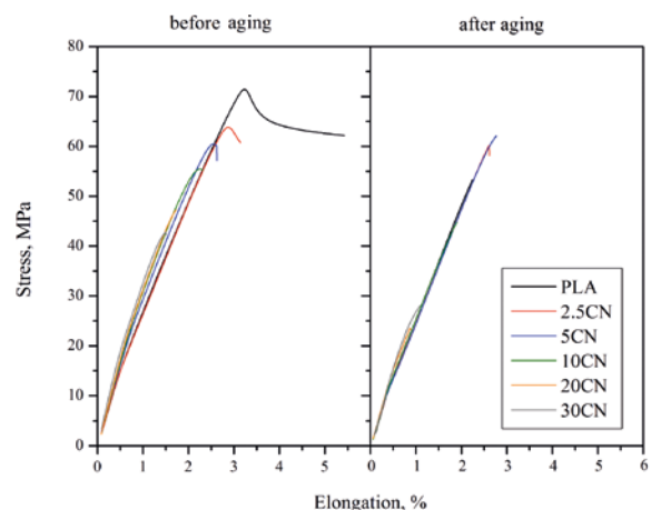
Fig. 3. Stress-strain curves of selected PLA and composite samples before and after aging process
