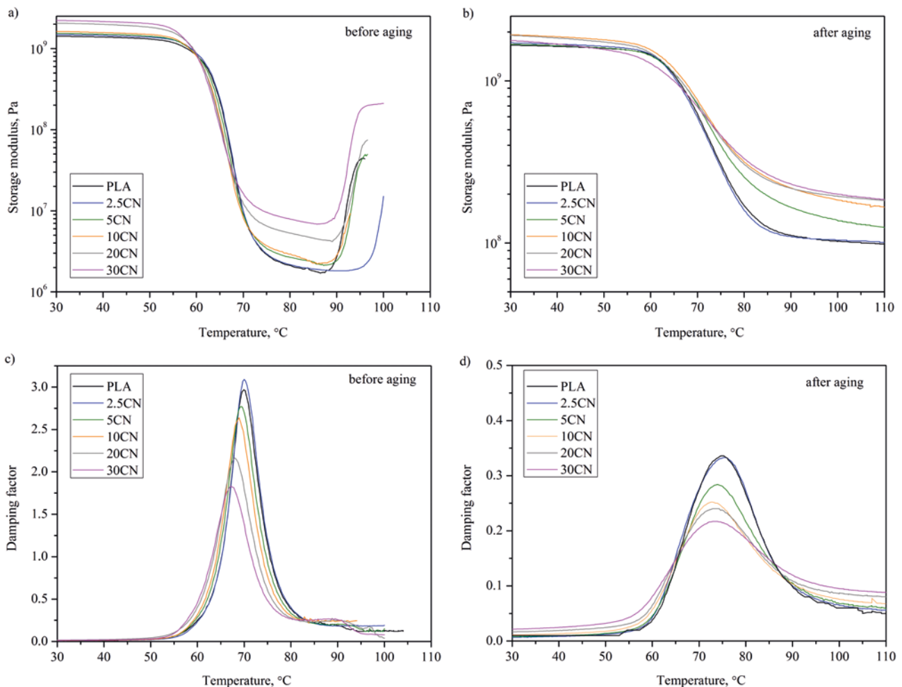
Fig. 4. a, b) Storage modulus ( G' ), c, d) damping factor ( \tan \delta ) of PLA and PLA composites before (a, c) and after (b, d) aging process
