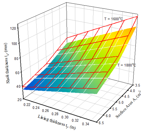
Fig. 12. Effect of temperature on hearth shell thickness t_s variation with lining thickness t_l and surface area A
