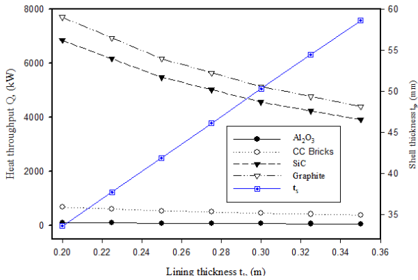
Fig. 11. Heat throughput Q and shell thickness t_s variation with lining thickness t_l for different refractory materials at constant surface area A = 6.5 \text{ m}^2 , T = 1800^\circ\text{C}
