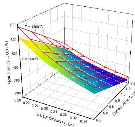
Fig. 14. Effect of temperature on heat throughput variation with hearth lining thickness and surface area of carbon composite bricks refractory
