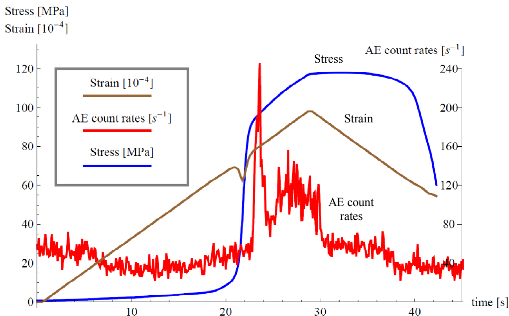
Fig. 3. Stress-strain curve, AE count rates and strain in interrupted compression test for Mg–AZ31 alloy at room temperature and strain rate of 0.00035 1/s
