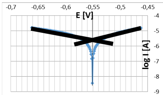
Fig. 3. Potentiodynamic research of MAO_2017_3
