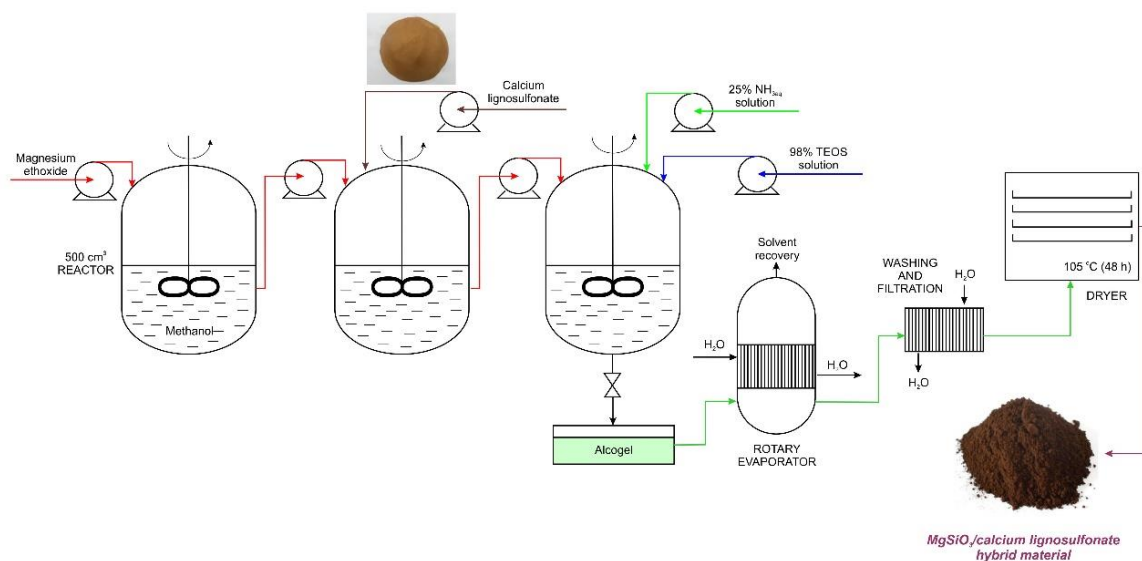
Fig. 1. In situ sol-gel synthesis of MgSiO 3 /lignosulfonate hybrid material
