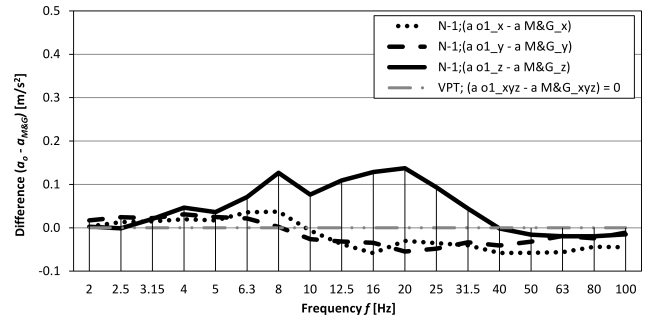
Fig. 8. Difference between measured vibration acceleration values for wheelchair W1 and Person 1 (in the directions X , Y , Z ) on the surface N-1 and the absolute threshold of vibration perception according to (MORIOKA, GRIFFIN, 2008).
