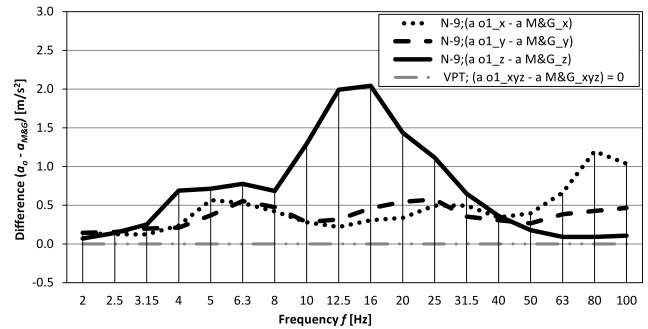
Fig. 9. Difference between measured vibration acceleration values for wheelchair W1 and Person 1 (in the directions X , Y , Z ) on the surface N-9 and the absolute threshold of vibration perception according to (MORIOKA, GRIFFIN, 2008).
