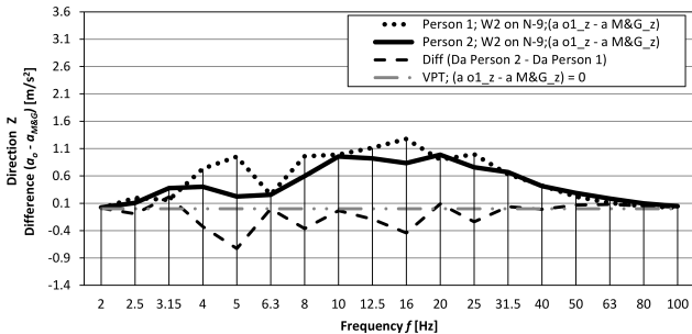
Fig. 17. Difference ( a_0 - a_{M\&G} ) for Persons 1 and 2 (for the direction Z) during the ride on the wheelchair W2 over the test surface N-9.
