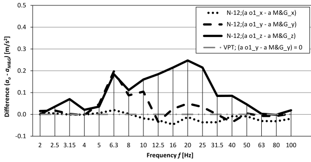
Fig. 11. Difference between accelerations measured for Person 2 and W1 (in the directions X , Y , Z ) on the test surface N-12 and the absolute threshold of vibration perception according to (MORIOKA, GRIFFIN, 2008).
