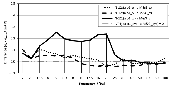
Fig. 10. Difference between accelerations measured for Person 1 and W1 (in the directions X , Y , Z ) on the test surface N-12 and the absolute threshold of vibration perception according to (MORIOKA, GRIFFIN, 2008).
