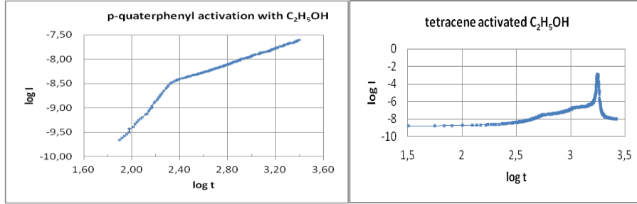
Fig. 1. Kinetics of the current for tetracene and p-quaterphenyl films vaporized with C_2H_5OH
