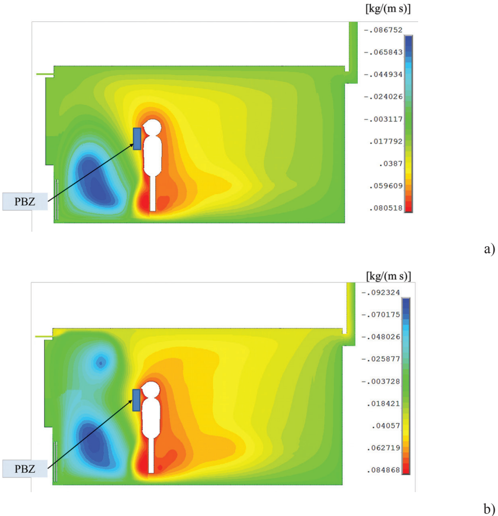
Fig. 12. Stream function \Psi [ \text{kg}/\text{m s} ] in indoor zone for resident located 1.7 m from window (location II) and for natural ventilation with exhaust ventilator: a) inlet air velocity of 0.05 m/s and b) inlet air velocity of 0.98 m/s
