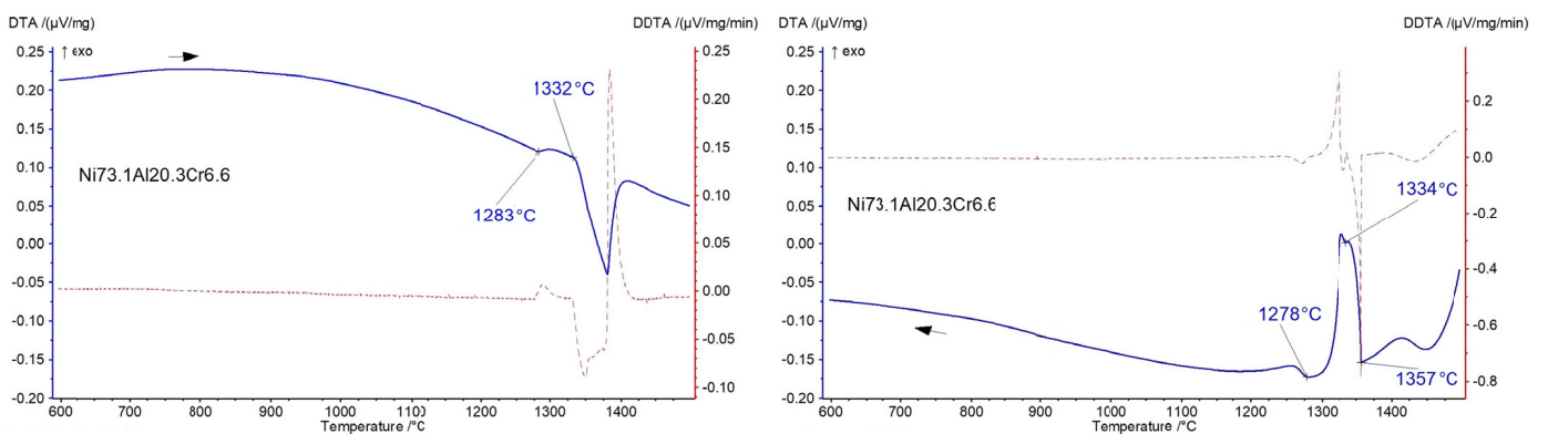
Fig. 9. DTA curves registered during heating (left) and cooling (right) of alloy Ni73.1Al20.3Cr6.6 (20°C/min)
