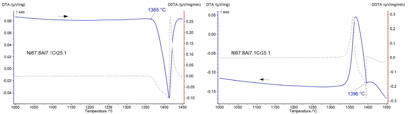
Fig. 4. DTA curves registered during heating (left) and cooling (right) of alloy Ni67.8Al7.1Cr25.1 (20°C/min)
