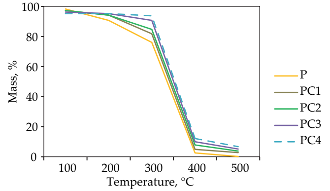
Fig. 6. TGA curves of PLA biocomposites
