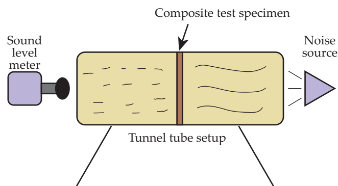
Fig. 1. Sound test impedance tube
