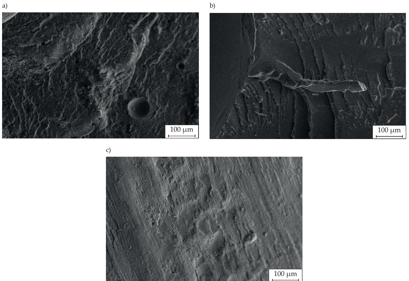
Fig. 7. SEM images of: a) PC4, b) PC3, c) PCG2
