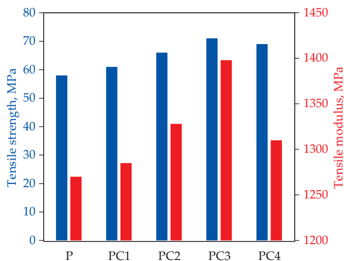
Fig. 2. Tensile strength and modulus of PLA biocomposites
