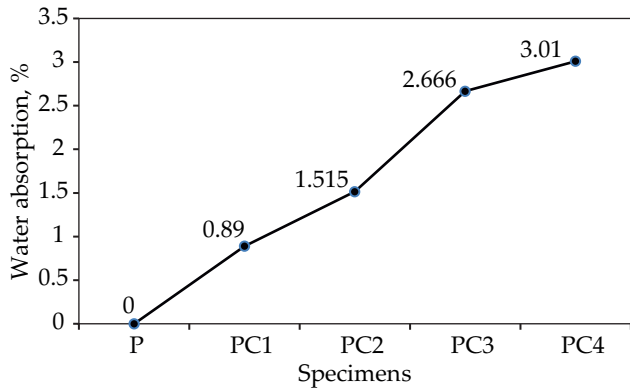
Fig. 5. Water absorption of PLA biocomposites
