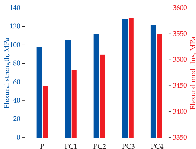
Fig. 3. Flexural strength and modulus of PLA biocomposites
