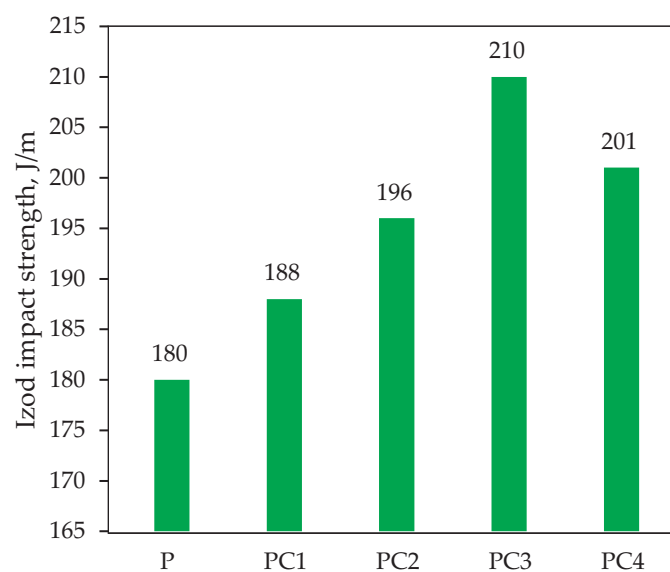
Fig. 4. Impact strength of PLA biocomposites
