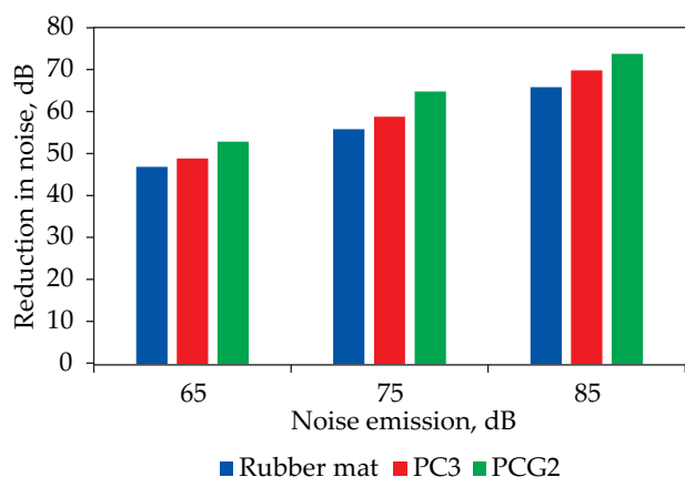
Fig. 8. Noise damping test analysis of rubber mat, PC3, and PCG2 biocomposites
