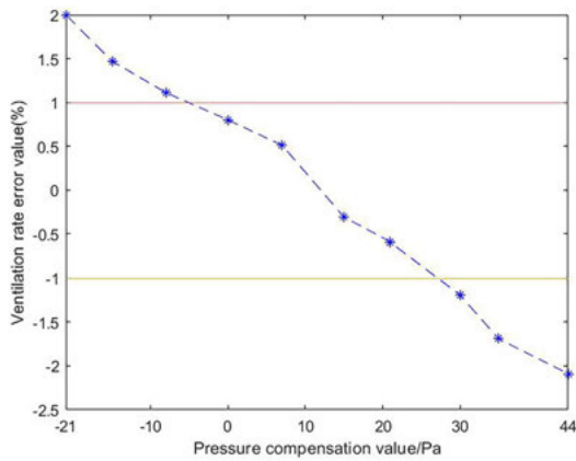
Fig. 7. Relationship between the experimental and verification values for the standard bar with a 58.83% ventilation rate.
