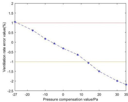
Fig. 8. Relationship between the experimental and verification values for the standard bar with a 71.95% ventilation rate.
