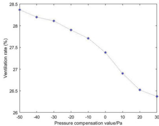
Fig. 4. Ventilation rate curve under different pressure differences.
