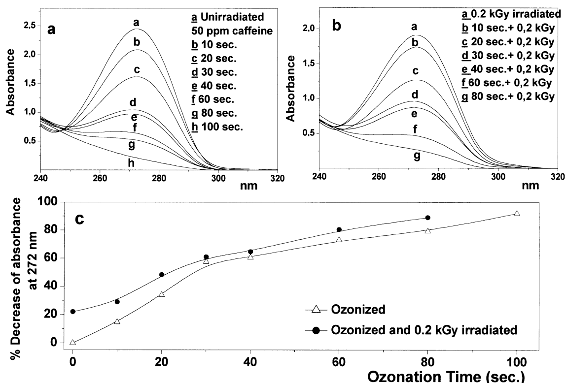
Fig. 2. Variation of the decrease of absorbance of 50 ppm caffeine as a function of ozonation time at 272 nm (a) ozonized without irradiation, (b) ozonized and irradiated for 0.2 kGy; (c) percent decrease in absorbance value.
