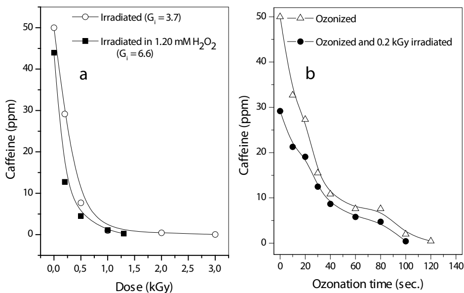
Fig. 4. Change in the amount of remaining caffeine in the treated aqueous samples as a function of (a) irradiation dose and (b) ozonation time. Analytical results were performed by GC/MS.
