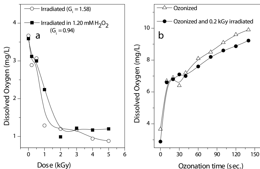
Fig. 6. Change in amounts of dissolved oxygen for caffeine solutions (50 ppm) as a function of (a) irradiation dose and (b) ozonation time.
