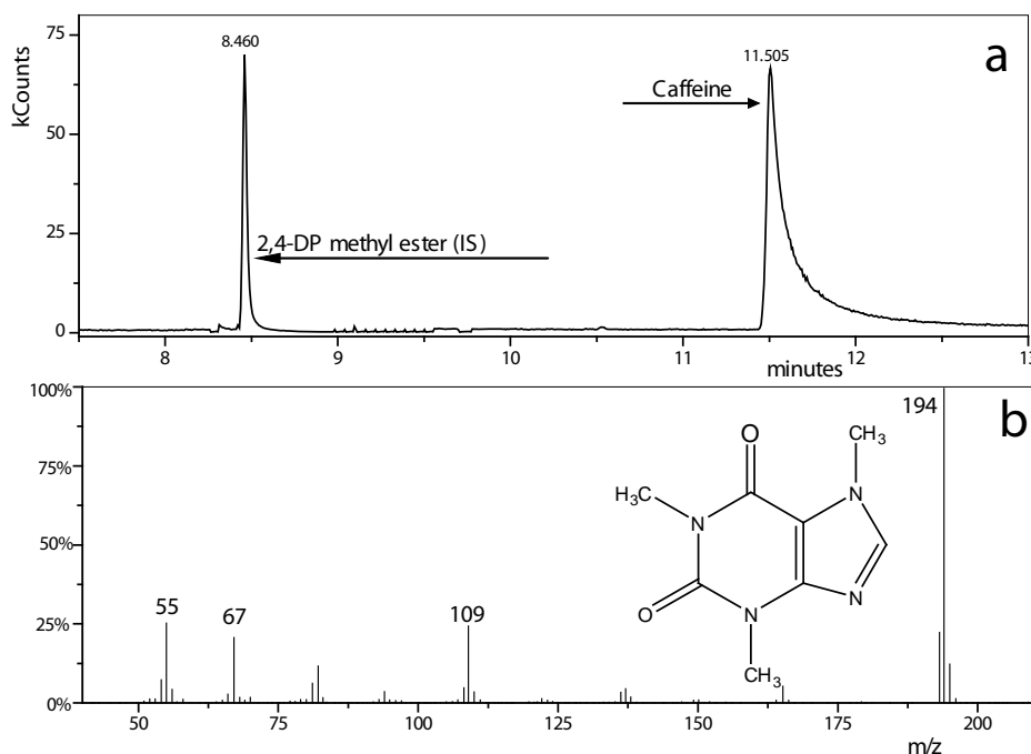
Fig. 3. (a) Gas chromatogram of caffeine (25 ppm) and 2,4-DP methyl ester as IS (20 ppm), (b) mass spectrum of caffeine.
