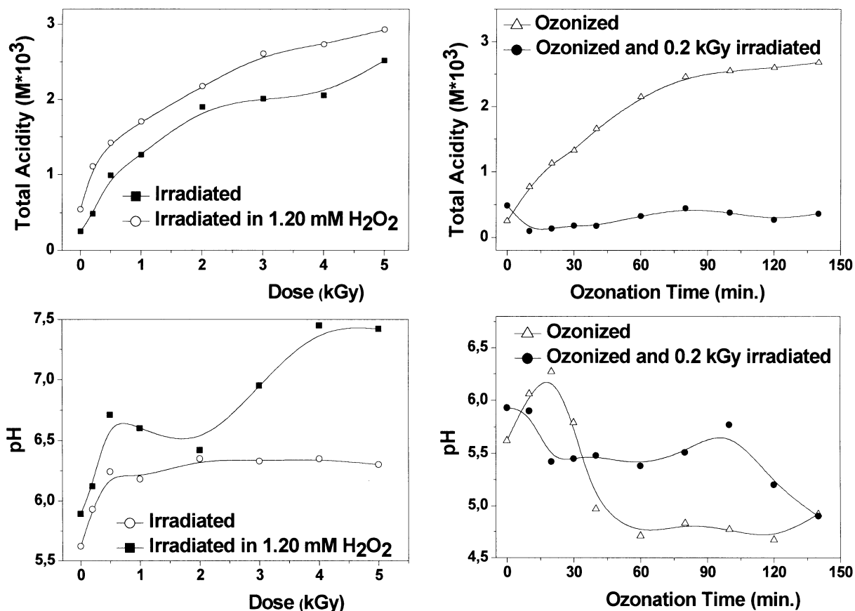
Fig. 5. Change in acidity and pH of caffeine solution (50 ppm) as a function of irradiation dose and ozonation time.
