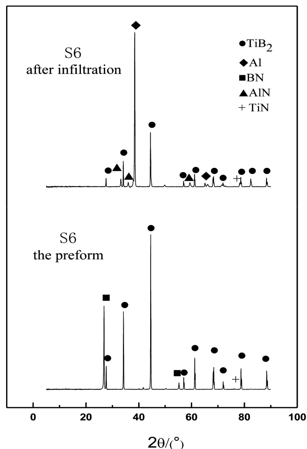
Fig. 1. XRD patterns of the S6 [Ti+BN] preform and the S6 composite material
