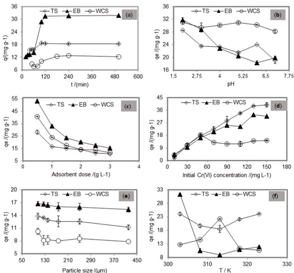
Figure 6. Cr(VI) removal capacity of TS, EB and WCS (a) contact time, (b) pH, (c) adsorbent dose, (d) initial metal concentration, (e) particle size (f) temperature. (Operating conditions except the variable parameter, initial Cr(VI) concentration 50 mg L -1 , pH 5.5, T 30°C, adsorbent dose 0.05 g L -1 , agitation speed 220 rpm, particle size 420 μm, equilibrium time for TS (100 minutes), EB (120 minutes), WCS (180 minutes))
