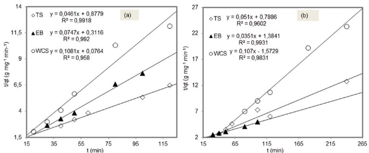
Figure 8. Pseudo-second order plot for Cr(VI) adsorption onto TS, EB and WCS at initial concentration of 50 \text{ mg L}^{-1} (a) and 70 \text{ mg L}^{-1} (b)
