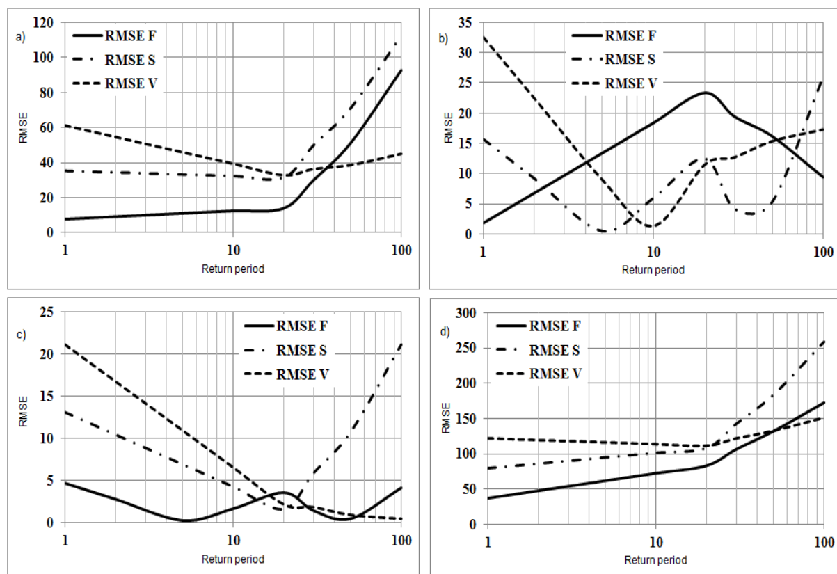
Fig. 10. Criterion of root mean squared error ( RMSE ) between local model and Q-d-F reference model for stations: a) Bir Ouled Tahar, b) Larabaa Ouled Fares, c) Tikazel, d) Sidi Akkacha; F, S, V as in Fig. 9; source: own study
