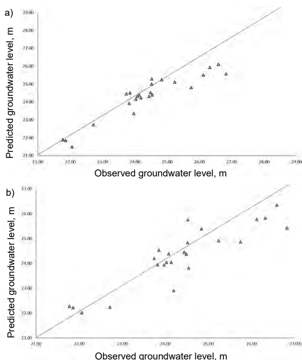
Fig. 7. Scatter plot of W303 comparing observed and simulated target values by best ELM model (a) and SVM model (b) in testing phase for one-month lead time; source: own study
