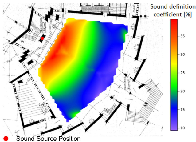
Fig. 12. Distribution of the definition coefficient D_{50} , the church of the VM.
