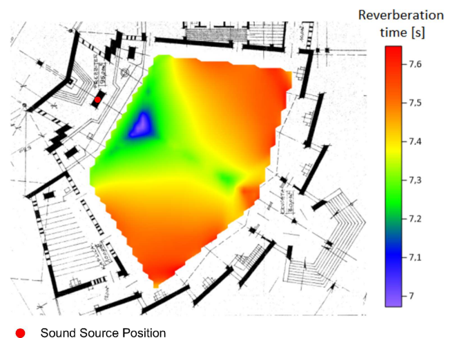
Fig. 11. Distribution of reverberation time T_{30} , the church of the VM.
