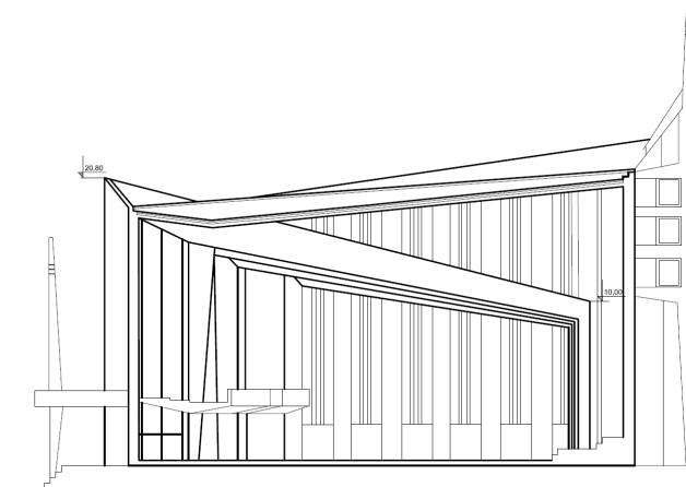
Fig. 9. The church of the Victorious VM, vertical section.
