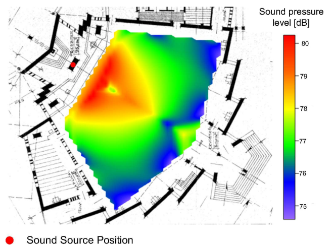
Fig. 10. Distribution of sound pressure level SPL, the church of the VM.
