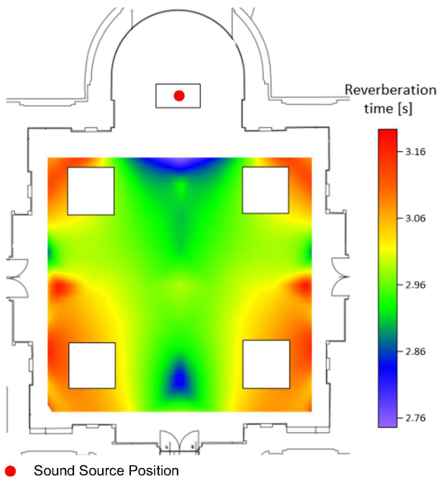
Fig. 3. Distribution of reverberation time T_{30} , St. James's Church.
