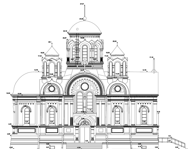
Fig. 1. St. James's Church, north elevation.
