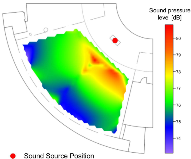
Fig. 6. Distribution of sound pressure level SPL, St. Hyacinth's Church.
