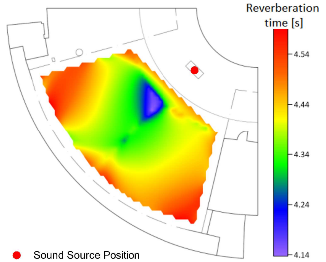
Fig. 7. Distribution of reverberation time T_{30} , St. Hyacinth's Church.
