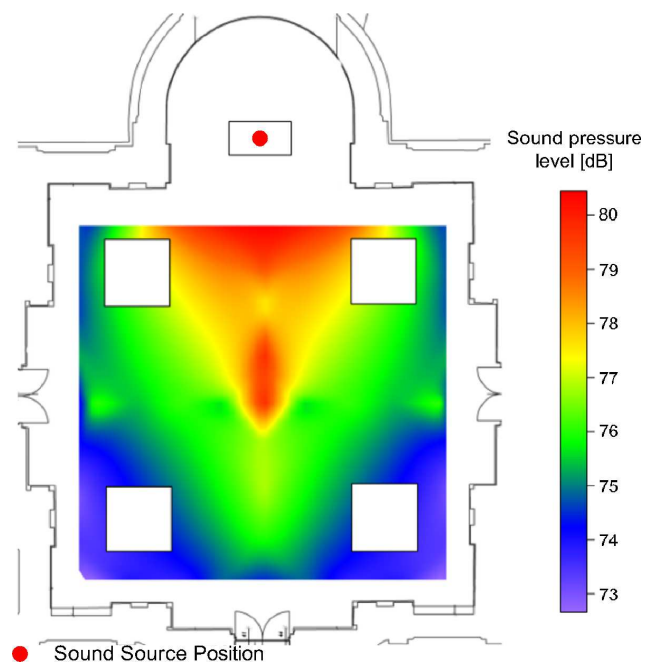
Fig. 2. Distribution of sound pressure level SPL, St. James's Church.
