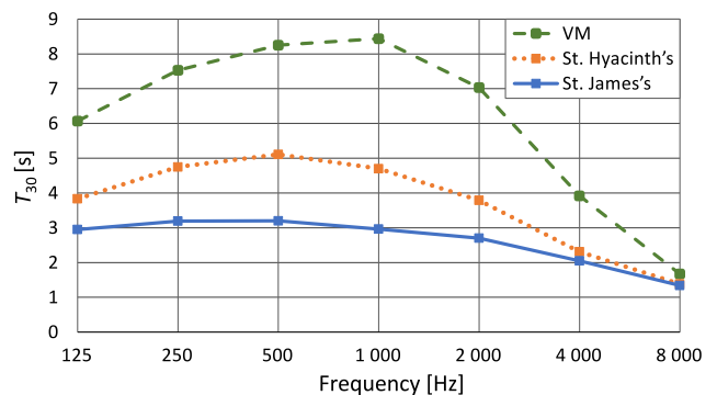
Fig. 13. Average reverberation time T_{30} as a function of frequency in the investigated temples.
