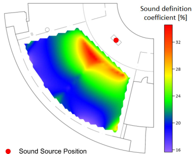
Fig. 8. Distribution of definition D_{50} , St. Hyacinth's Church.
