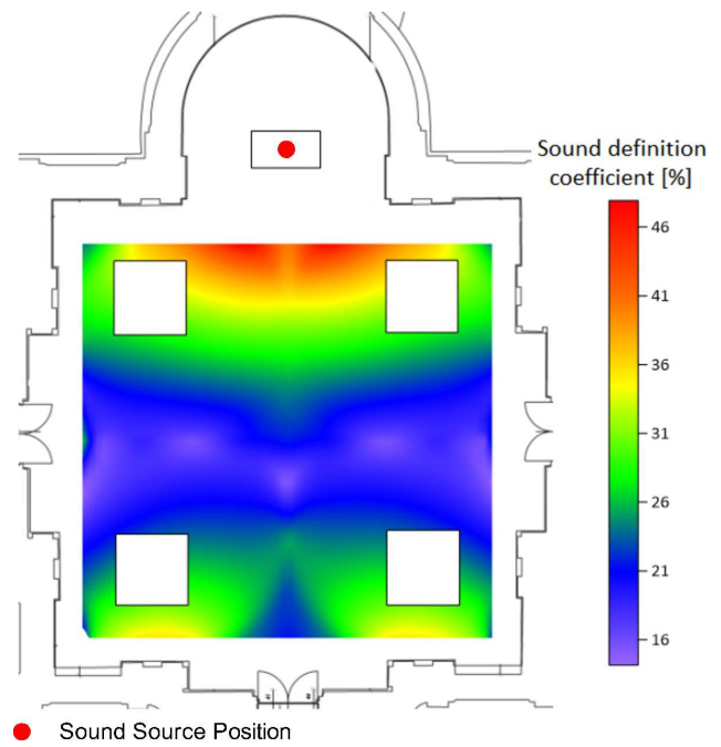
Fig. 4. Distribution of the definition D_{50} , St. James's Church.
