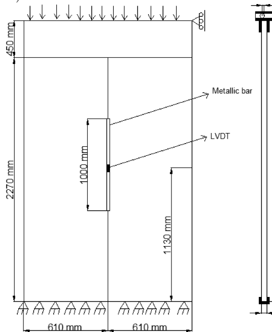
Fig. 2. Set-up of the apparatus used on the static experimental tests; a) photograph of the experimental set-up for the static compression test; b) schematic representation for the compression test.
