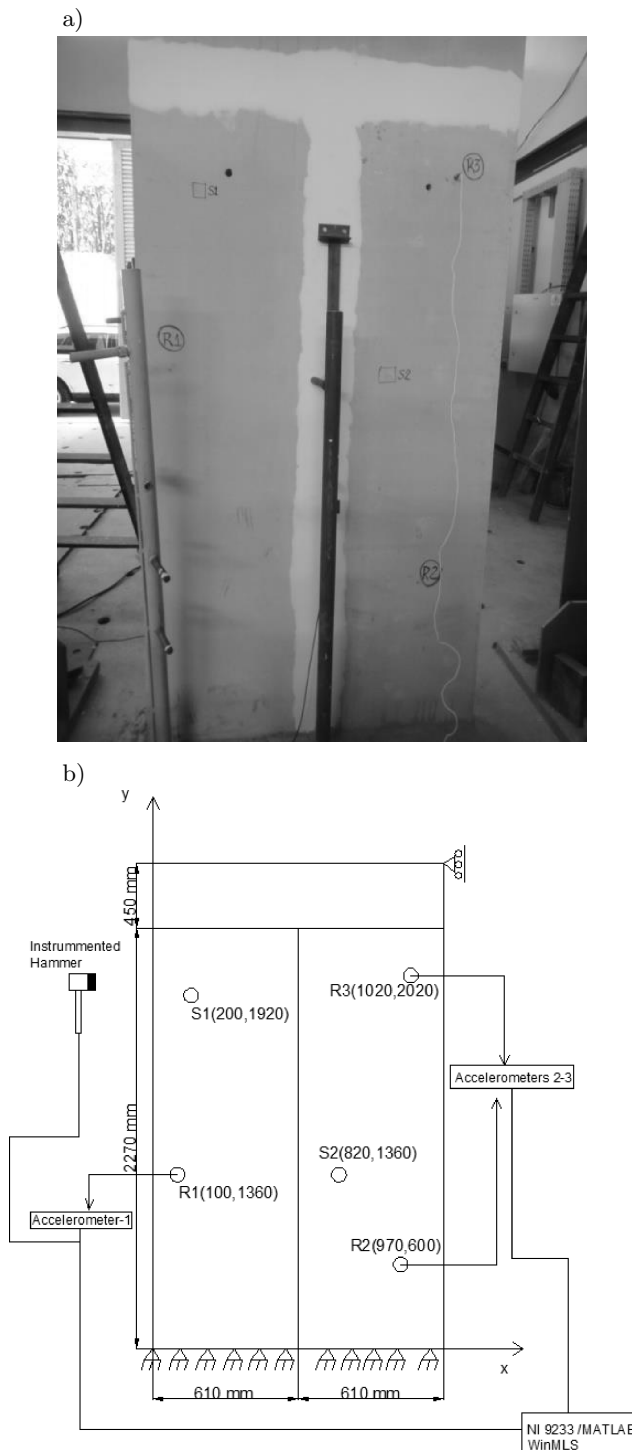
Fig. 3. Set-up of the apparatus used on the dynamic tests; a) photograph of the experimental set-up for the dynamic test; b) schematic representation.
