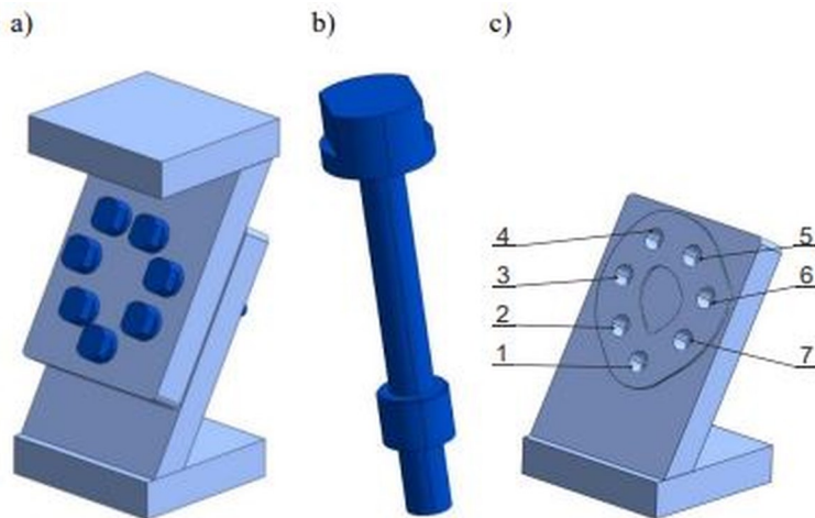
Fig. 1. Model of the connection: (a) model 3D, (b) model 3D of the single fastener, (c) outline of the surface at the contact of the joined plates and assumed numbering of the bolts
