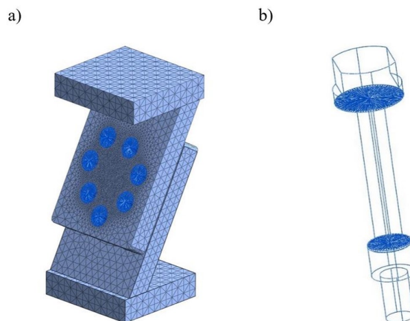
Fig. 2. FE-model of the bolted connection: (a) entire connection, (b) single fastener
