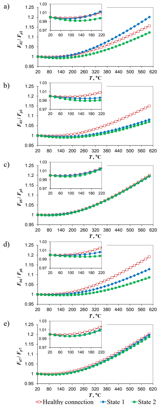
Fig. 3. Distributions of bolt forces in the connection pretensioned according to the queue No. 3: a) bolt No. 2, b) bolt No. 3, c) bolt No. 5, d) bolt No. 6, e) bolt No. 7
