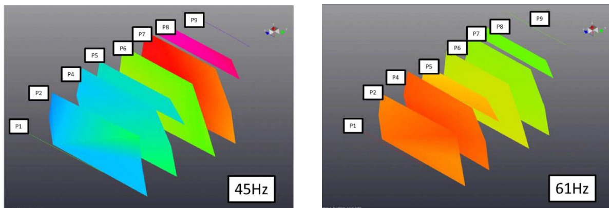
Fig. 5. Experimental cavity modal analysis of the studied vehicles.
