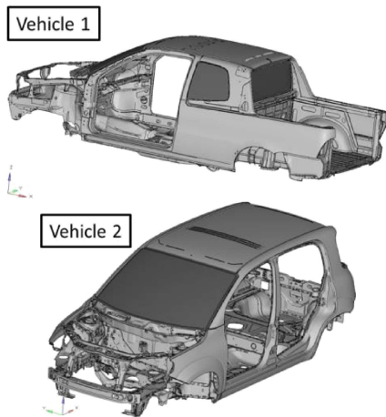
Fig. 13. Numerical models in the body in white version.
