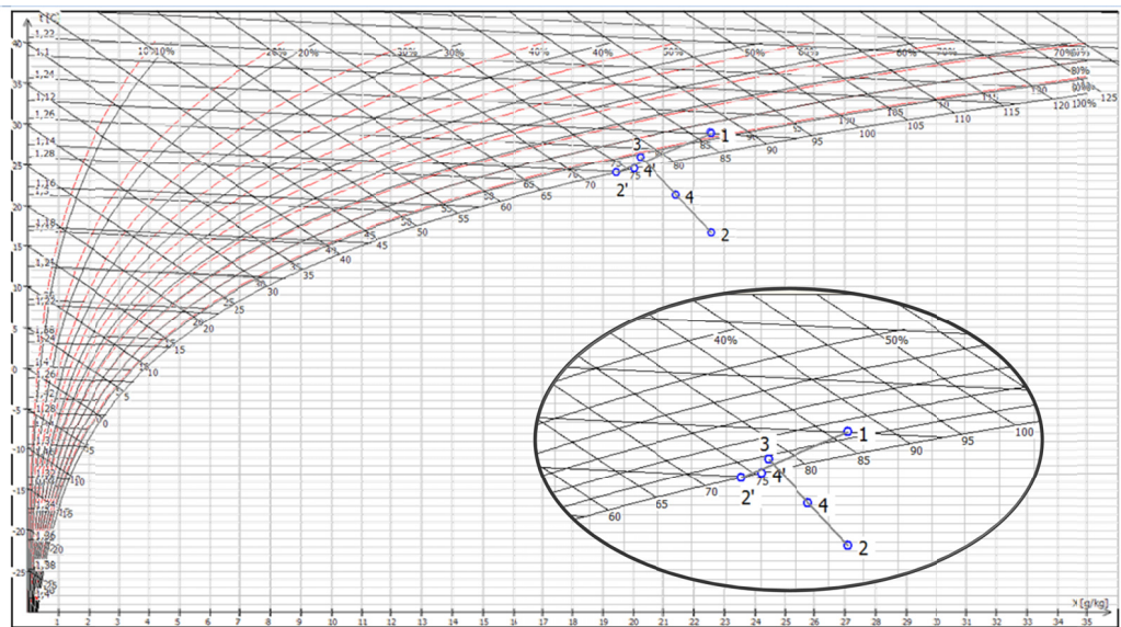
Fig. 4. Cooling and mixing transitions of the air streams in section 1-4 of the exhausting shaft
