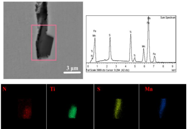
Fig. 2. TiN inclusion wrapped by MnS in wire rod
