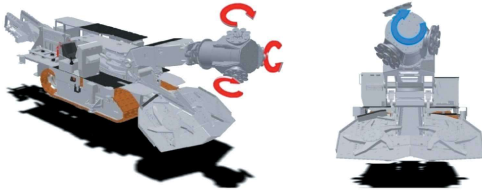
Fig. 3. Kinematic capabilities of new head solution mounted on roadheader KR 150 [3]
