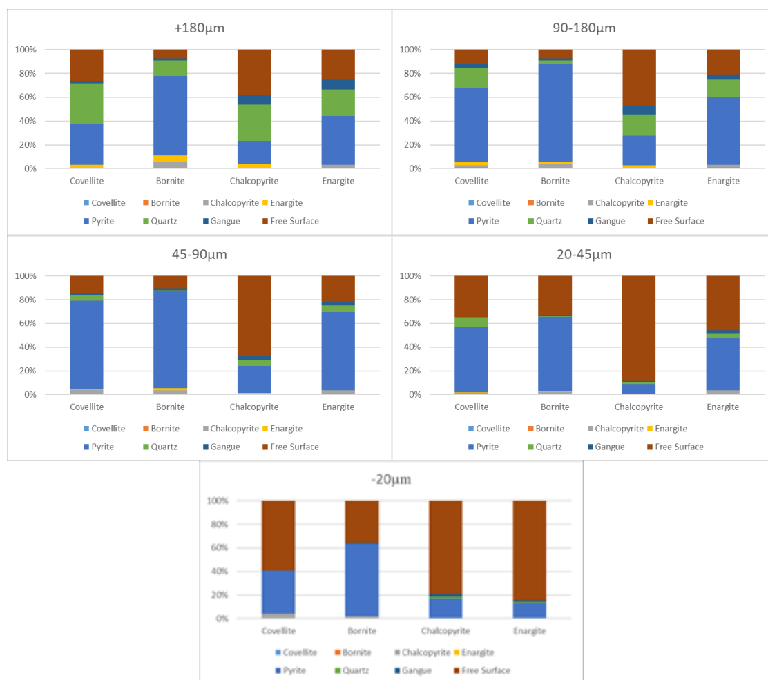
Fig. 6. Copper mineral association in the tested size fractions
