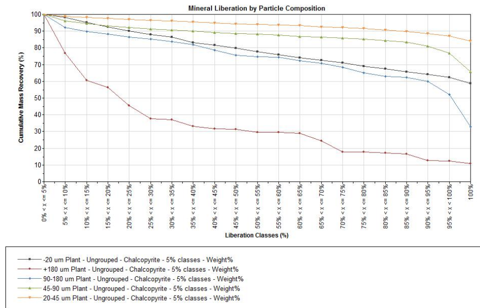
Fig. 8. Chalcopyrite mineral liberation by particle composition
