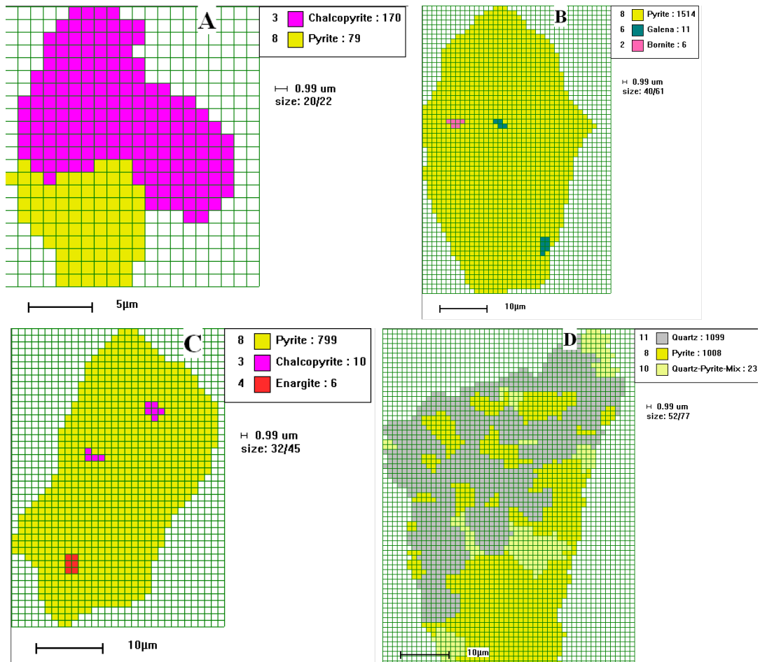
Fig. 10. Particle images as given by the MLA
