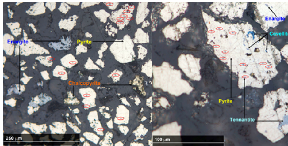
Fig. 7. Optical view of 45-90 \mu\text{m} Cu-selective scavenger feed (left) and scavenger tailings (right) (micro inclusions)
