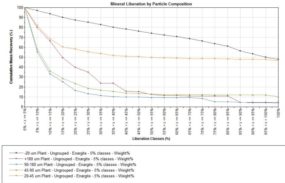
Fig. 9. Enargite/tennantite mineral liberation by particle composition
