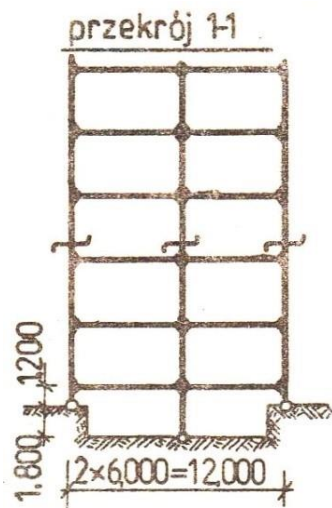
Fig. 5. 1-1 cross section of Lipsk III type building [10]
