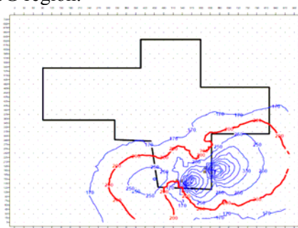
Fig. 5. The maximum of percentile S99.8 for NO 2
