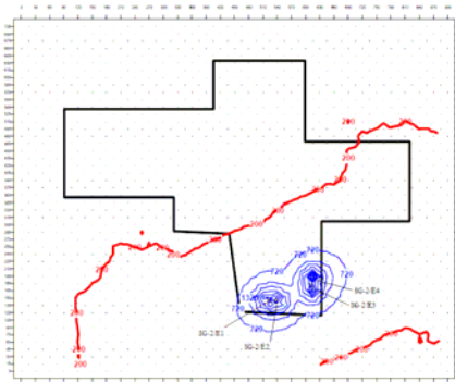
Fig. 4. The distribution of the contour lines of NO 2 dispersion for a maximum 1-hour concentration
