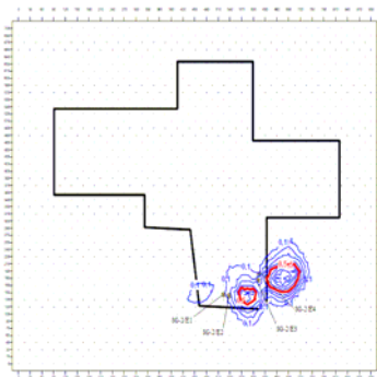
Fig. 3. The incidence of reference value exceedance for SO 2 for a calendar year [%]
