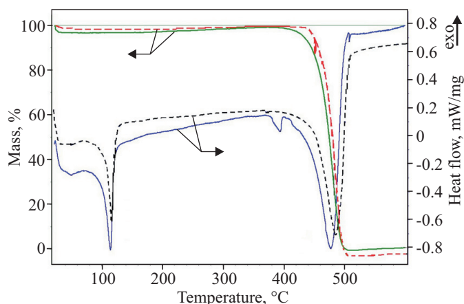
Fig. 5. TG and DSC thermograms with registered transitions registered for PE-LD (green – TG, blue – DSC) and PE-LD + 5 % FA (15–30 \mu\text{m} , red – TG, black – DSC) samples
