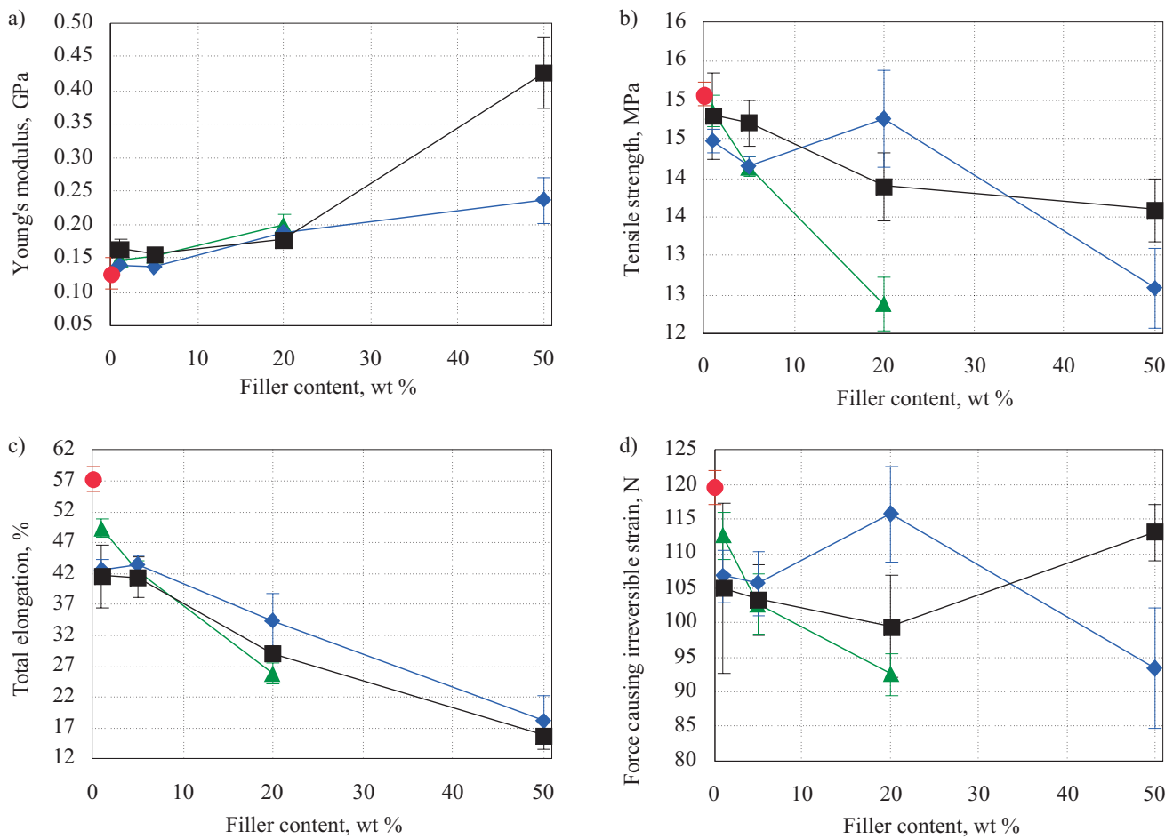
Fig. 2. The influence of the FA content and FA grain size (black — 0–15 \mu\text{m} , blue — 15–30 \mu\text{m} , and green — 30–60 \mu\text{m} , red — pure PE-LD) on: a) average Young's modulus ( E ), b) average tensile strength, c) average total elongation, d) average force causing irreversible strain
