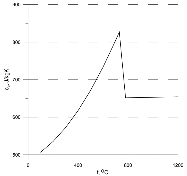
Fig. 3. Specific heat [2]
