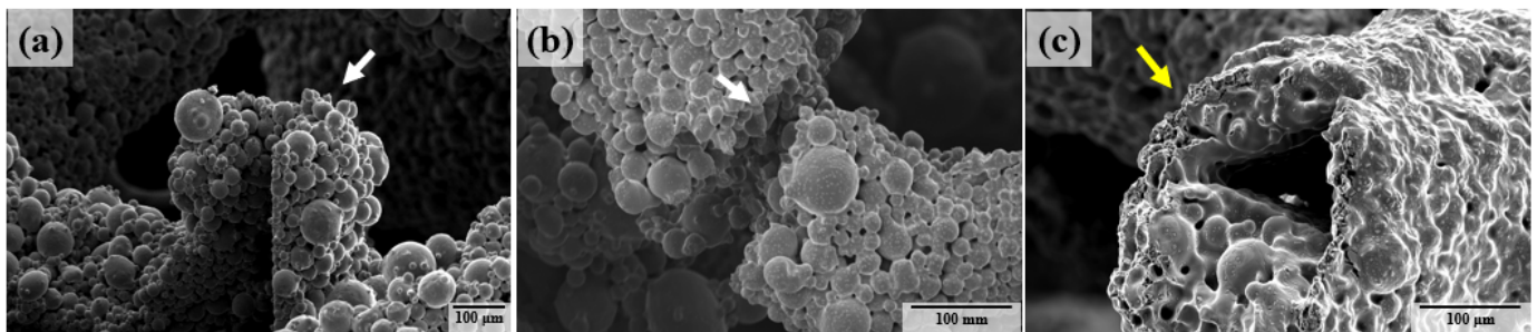
Fig. 6. SEM image of compressed foams: 1200 foam (a), 1250 foam (b) and 1300 foam (c)
