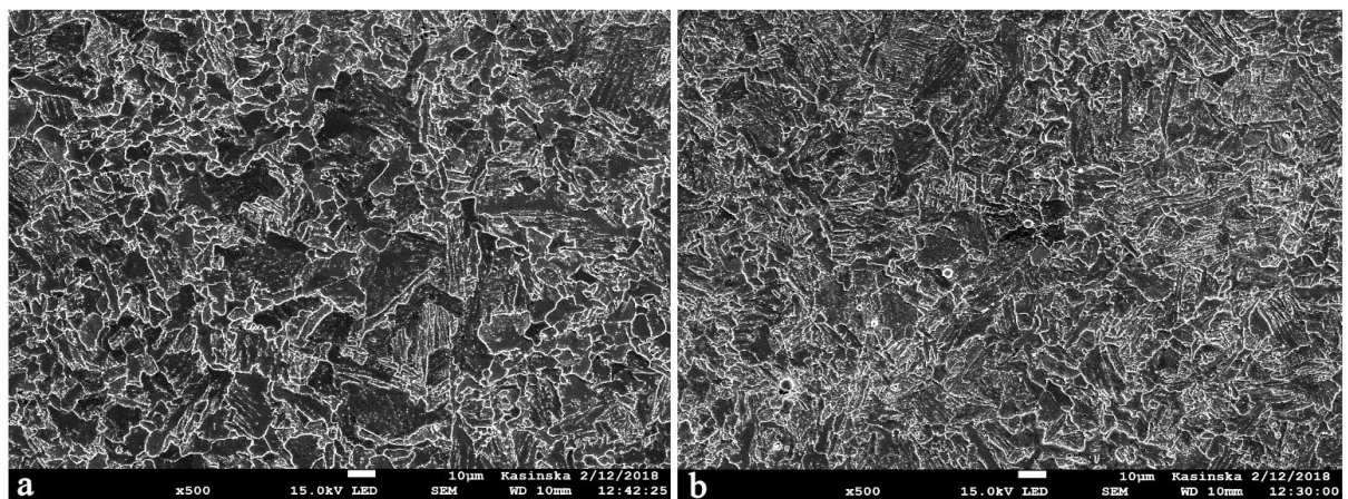
Fig. 6. Microstructure of heat-treated cast steel, a) without REMs, b) with the REM additive, SEM; nital etched
