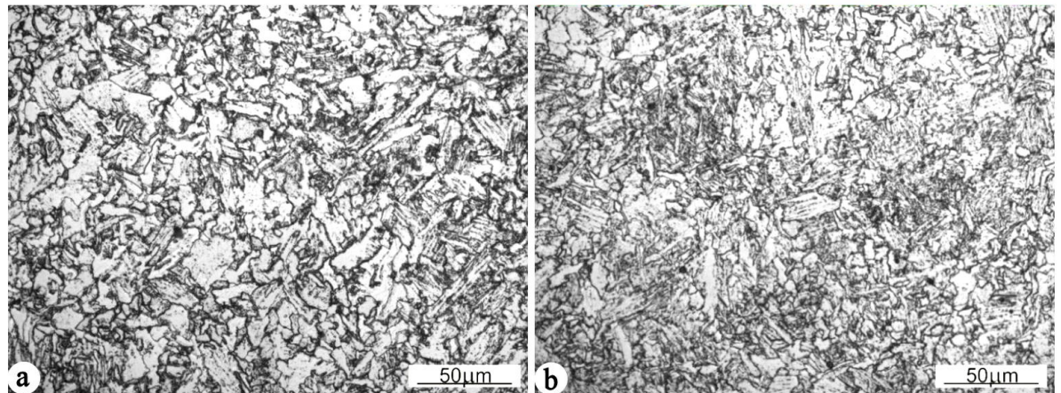
Fig. 5. Microstructure of heat-treated cast steel, a) without REMs, b) with the REM additive, LM; nital etched
