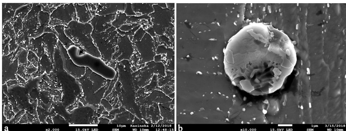
Fig. 7. Microstructure of cast steel with visible non-metallic inclusions, a) without REMs, b) with the REM additive, SEM; pickled with nital.
