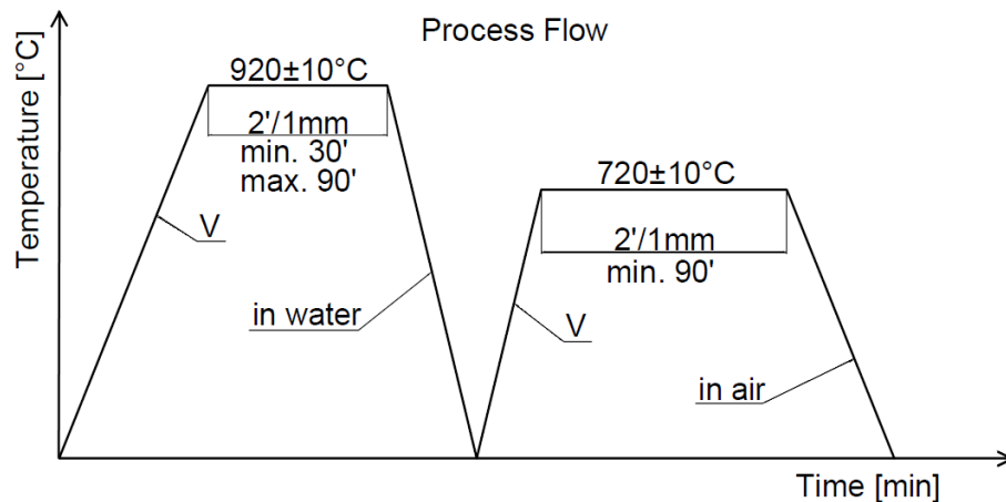
Fig. 2. Process flow of heat treatment
