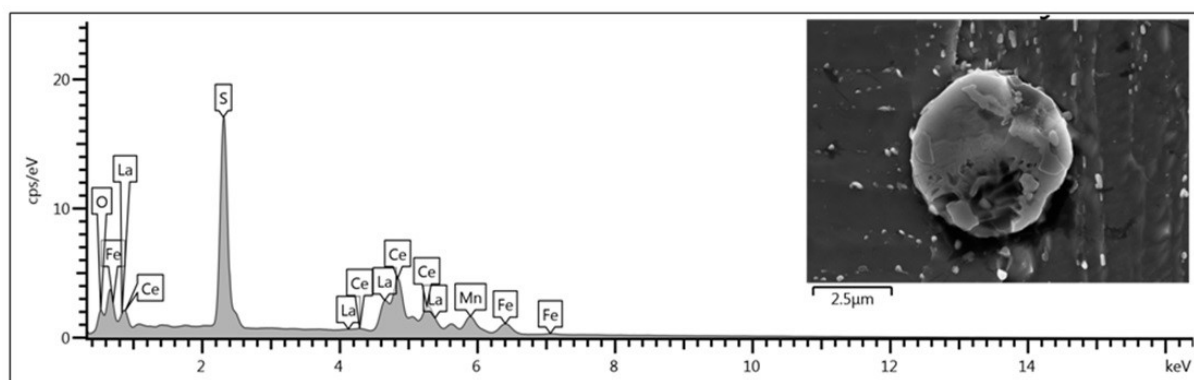
Fig. 9. Characteristic X-ray spectrum of a non-metallic inclusion in modified cast steel, SEM, EDS
