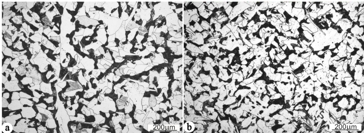
Fig. 4. Microstructure of as-cast steel, a) without REMs, b) with the REM additive, LM; nital etched
