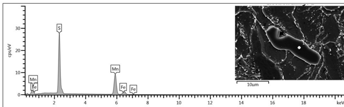
Fig. 8. Characteristic X-ray spectrum of a non-metallic inclusion in modified cast steel, SEM, EDS
