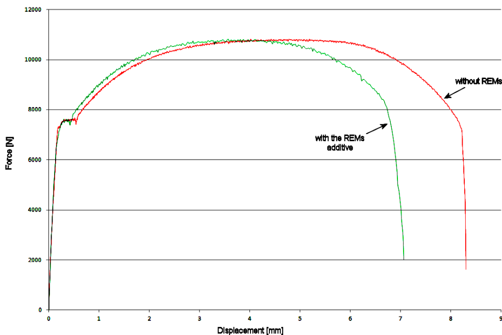
Fig. 3. Examples of tensile test charts for cast steel without REMs and with the REM additive
