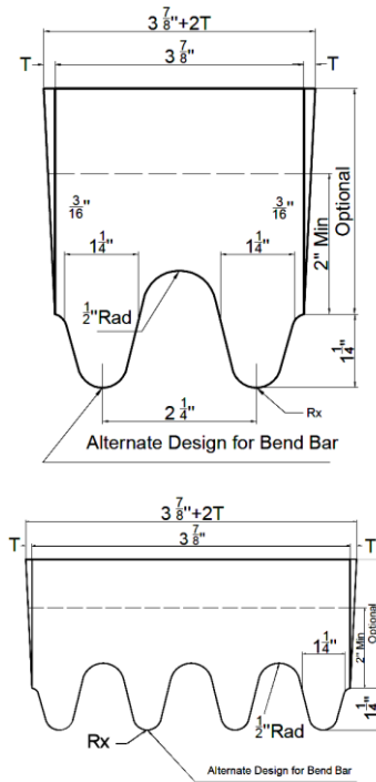
Fig. 1. Scheme of test ingots in compliance with ASTM A370-77
