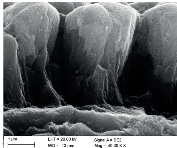
Fig. 1. Fracture surface of Ti(C,N) coatings
