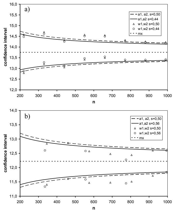
Fig. 7. Austenite grain size confidence interval values ( w_1 , w_2 ) and the expected values ( a_1 , a_2 ) as function of chord number n for the data-sets: a) L15 ( s_{\ln x} = 0,44 and s_{\ln x} = 0,50 ) and b) L11: s_{\ln x} = 0,56 and s_{\ln x} = 0,50 ; s = s_{\ln x}
