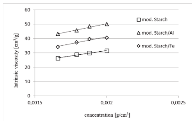
Figure 5. Dependence of reduced viscosity on concentration of a modified starch and hybrids modified starch/Me 3+ solutions
