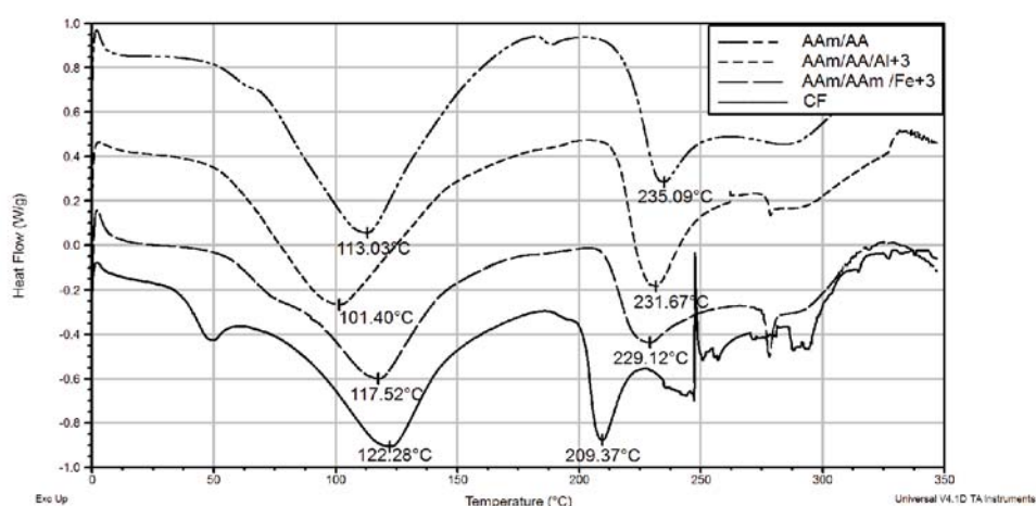
Figure 3. The DSC thermographs acrylamide copolymers-AAm/AA, by trivalent cations copolymers: AAm/AA/ \text{Al}^{+3} , AAm/AA/ \text{Fe}^{+3} and commercial flocculant CF
