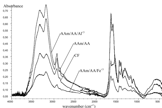
Figure 1. The FTIR spectra of the acrylamide copolymers-AAm/AA, modified by trivalent cations copolymers: AAm/AA/ \text{Al}^{+3} , AAm/AA/ \text{Fe}^{+3} and commercial flocculant CF
