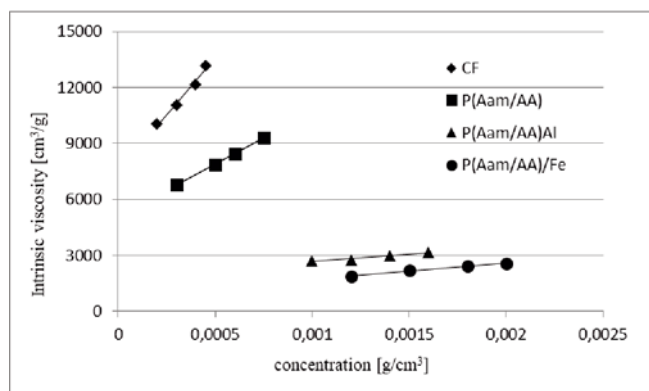
Figure 4. Dependence of reduced viscosity on concentration of an acrylamide copolymer-AAm/AA, hybrids AAm/AA/Me 3+ and commercial flocculant CF solutions
