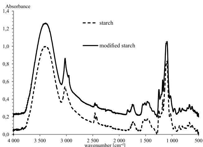
Figure 2. The FTIR spectra of the potato starch and modified starch by oxidation
