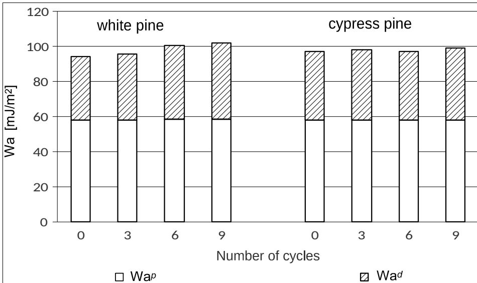
Fig. 4. Formation of the work of adhesion ( Wa ) and dispersion ( Wa^d ) and polar ( Wa^p ) shares for surface of various coloured lacquer systems formed on pine wood as a function of the number of thermal aging cycles
