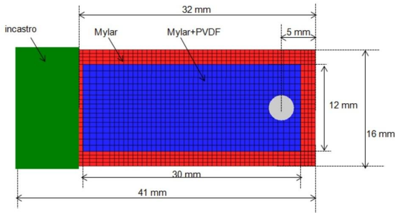
Fig. 11. FEM model of measurement specialties LDT1-028K
