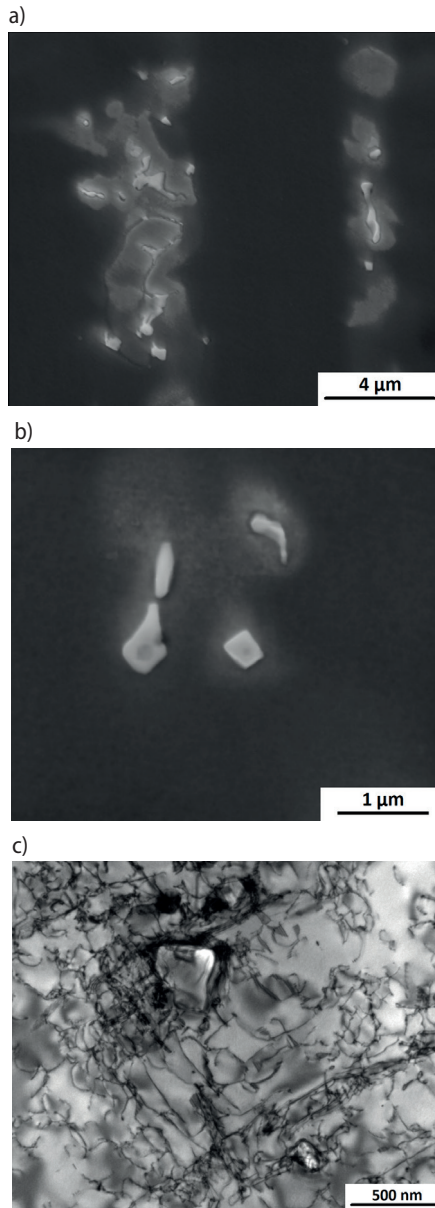
Fig. 2. SEM and TEM images of precipitates observed in Inconel 625 overlay: (a, b) SEM of Laves phase and carbide; c) BF-TEM of carbide
