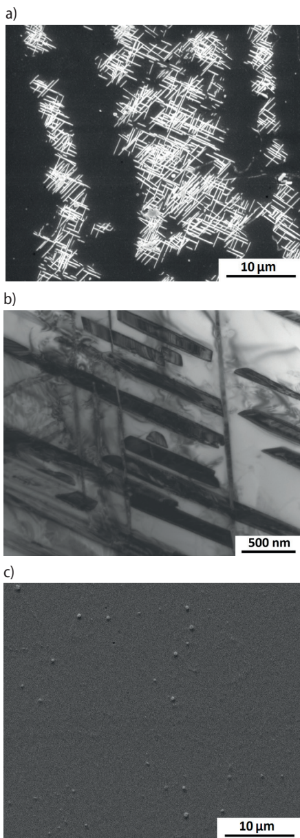
Fig. 3. Microstructure after annealing: a) 800°C (SEM); b) 800°C (BF-TEM); c) 1000°C (SEM)
