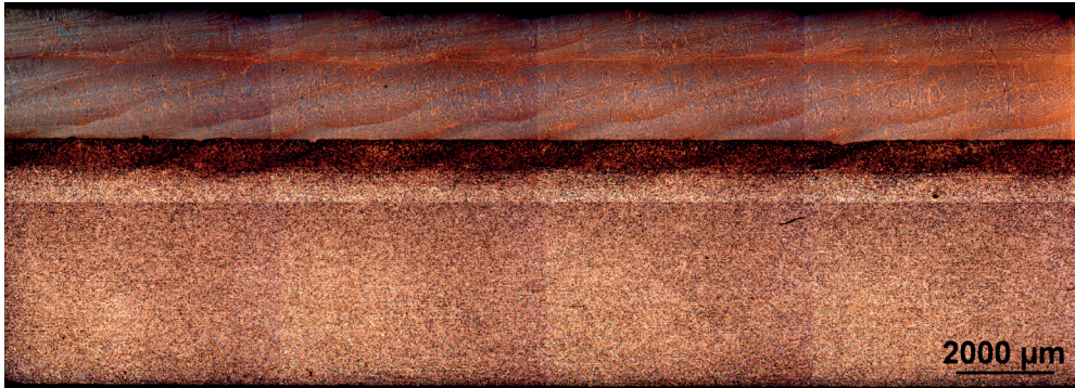
Fig. 1. Macrostructure of clad layer of Inconel 625 alloy
