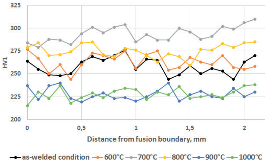
Fig. 5. Hardness distribution in weld overlay
