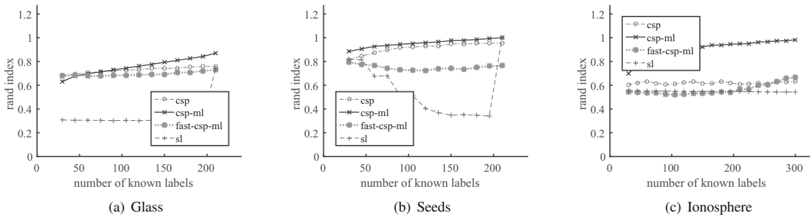
Fig. 3. Performance comparison of different constrained spectral clustering algorithms on a constrained data set with noise.
