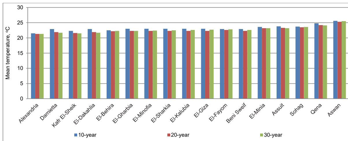
Fig. 3. Comparison between mean temperature values averaged over 10, 20 and 30 years; source: own study
