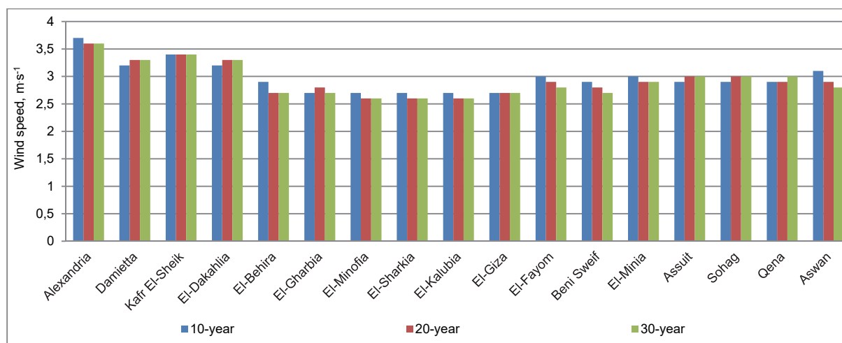
Fig. 4. Comparison between wind speed values averaged over 10, 20 and 30 years; source: own study
