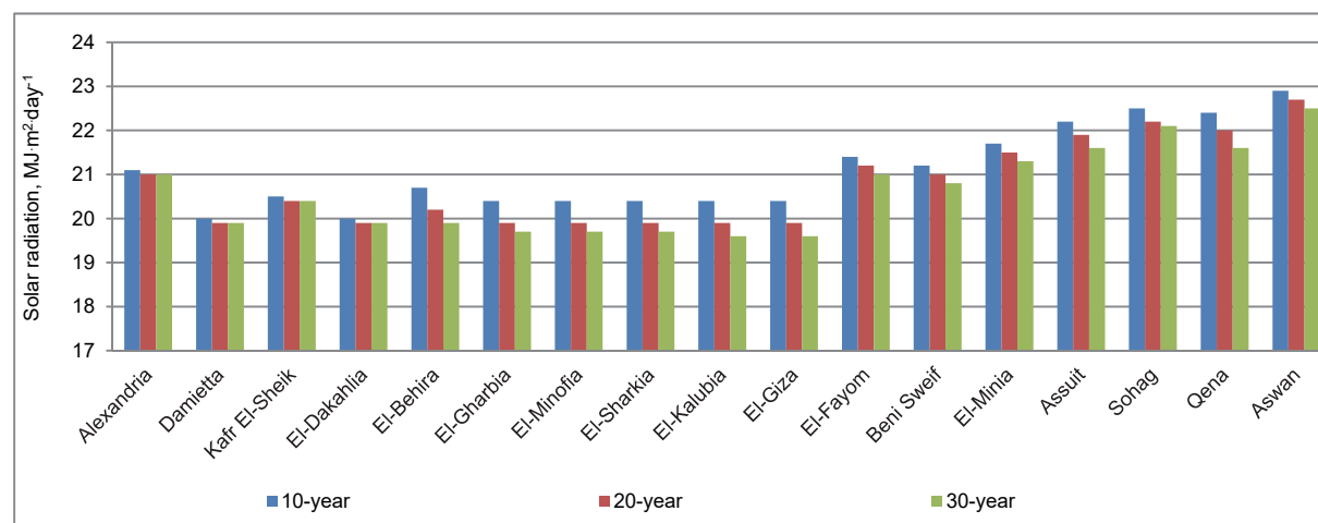
Fig. 2. Comparison between solar radiation values averaged over 10, 20 and 30 years; source: own study
