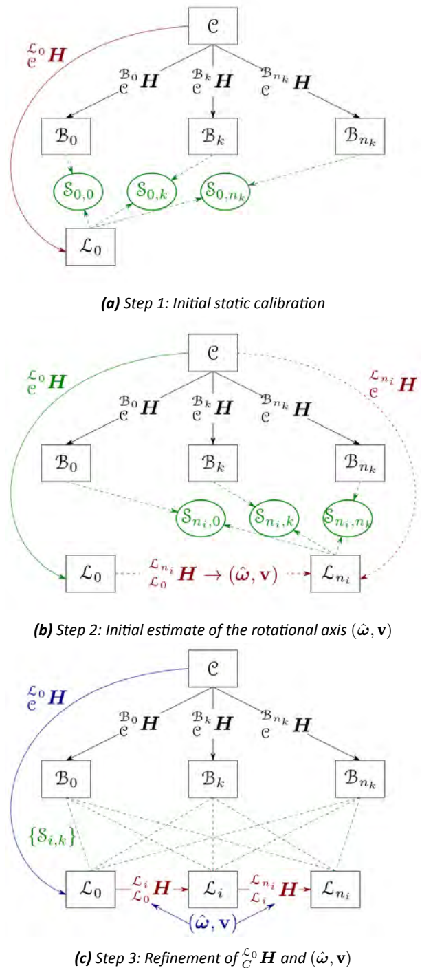
Fig. 4. Calibration Procedure
