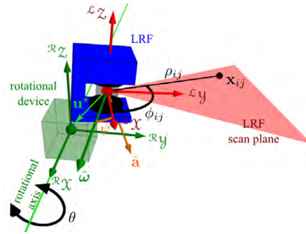
Fig. 2. Coordinate frames of the rotational device and the LRF. The axis of rotation of a rotating LRF relative to its mirror center has 4 degree of freedoms: 2 for the offset distance \mathbf{u}^* = [0, u_y^*, u_z^*]^T in the \mathcal{Y} - \mathcal{Z} plane of the LRF, and 2 for the unit vector \hat{\omega} in the direction of the rotational axis
