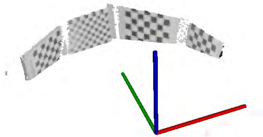
Fig. 10. Laser points with intensity values reconstructed after calibration, showing a rough outline of the scanned checkerboard patterns
