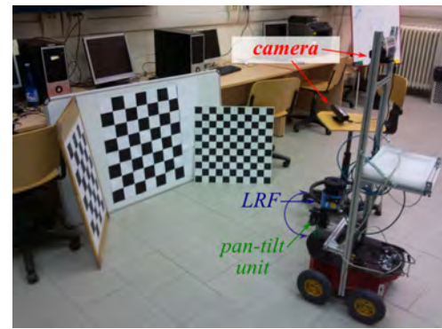
Fig. 3. Calibration setup: 3 or more planar calibration patterns are scanned by the rotating LRF and imaged by a static camera
