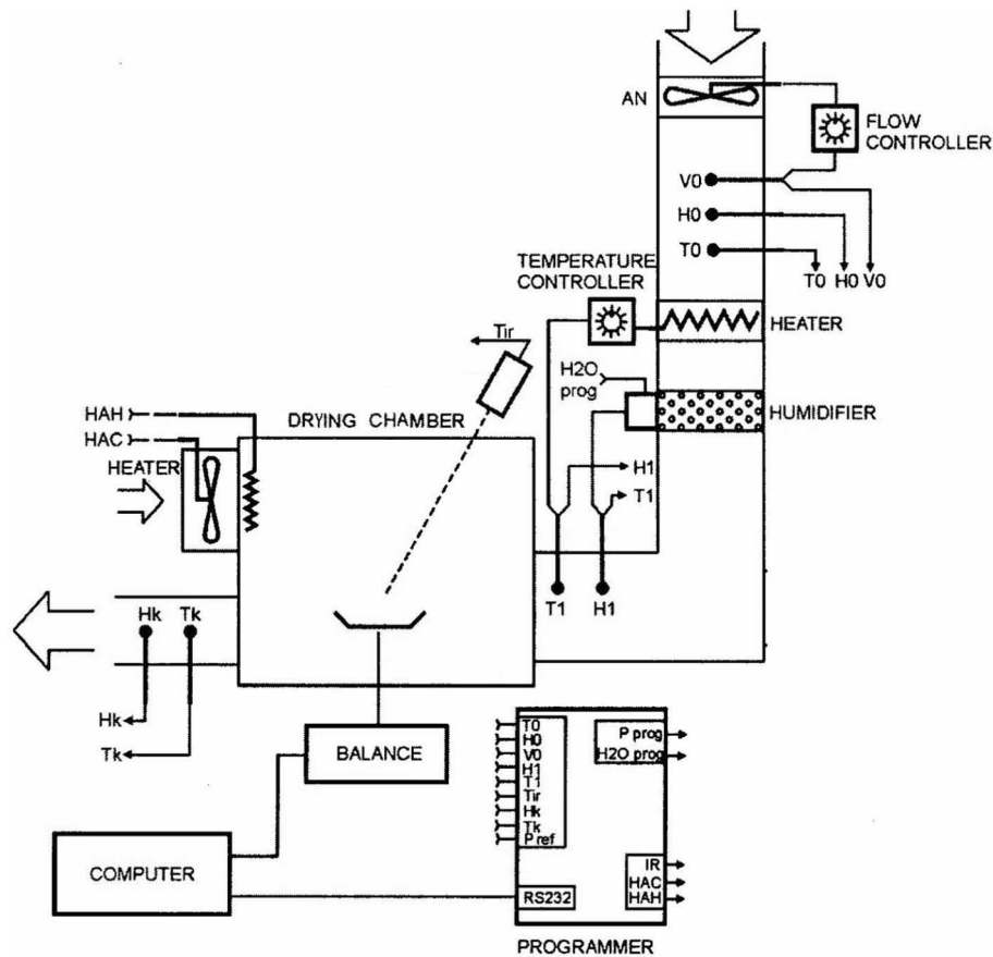
Fig. 1. Scheme of dryer (Kowalski and Rajewska, 2009)
