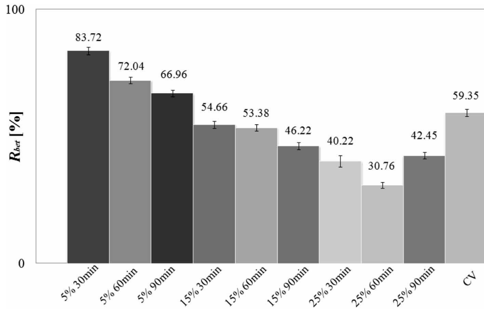
Fig. 5. Relative retention of betanin after CV samples and those treated with osmotic dehydration
