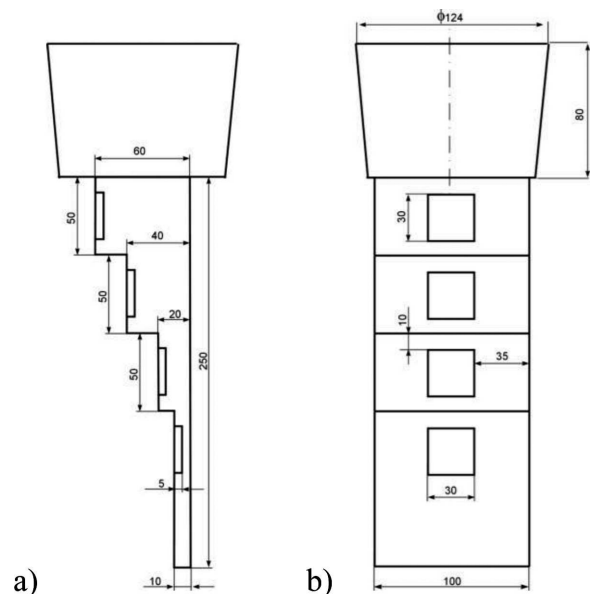
Fig. 1. The shape of experimental cast; a) section, b) sight
