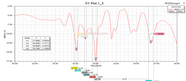
Fig. 17. Bandwidth analysis of optimized 2x2 optimized slotted rectangular patch array using RT6010
