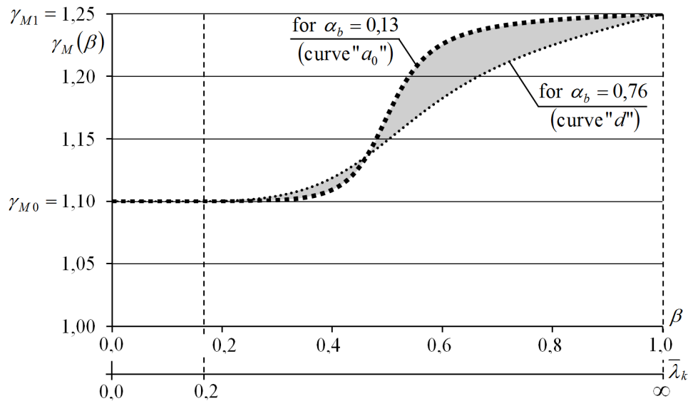
Fig. 3. Slenderness dependent partial resistance factor \gamma_M
