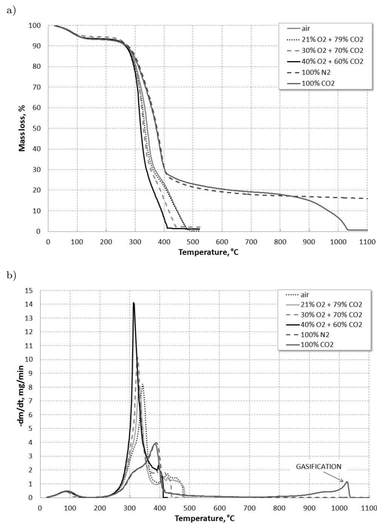
Figure 5: Thermogravimetric, TG, (a) and differential thermogravimetric, DTG, (b) curves for wooden biomass combustion and pyrolysis.
