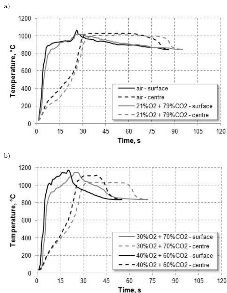
Figure 4: Temperature profiles for wooden biomass particle burned at 850 °C in various atmospheres: a) air and 21%O 2 /79%CO 2 , b) 30%O 2 /70%CO 2 and 40%O 2 /60%CO 2 .
