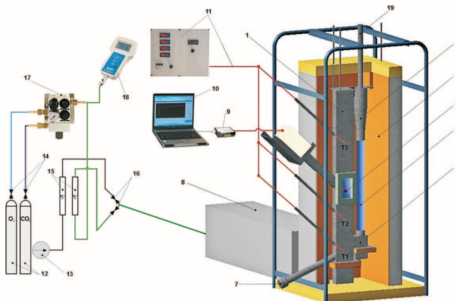
Figure 1: Schematic diagram of the experimental apparatus [2]: 1 – combustion chamber, 2 – cyclone, 3 – downcomer, 4 – loop seal, 5 – biomass particle, 6 – insulation, 7 – drain valve, 8 – preheater, 9 – card, 10 – computer, 11 – temperature control system, 12 – gas cylinders, 13 – air compressor, 14 – pressure regulators, 15 – rotameters, 16 – valves, 17 – mixer, 18 – gas analyser, 19 – ventilation duct, T1–T3 – S-type thermocouples.
