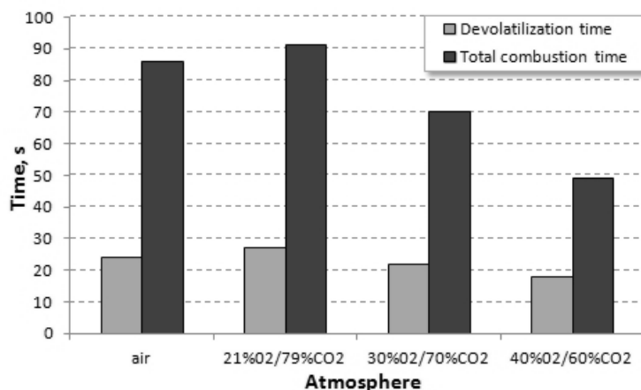
Figure 3: Devolatilization time and total combustion time for biomass particles burned in various atmospheres at 850 °C.
