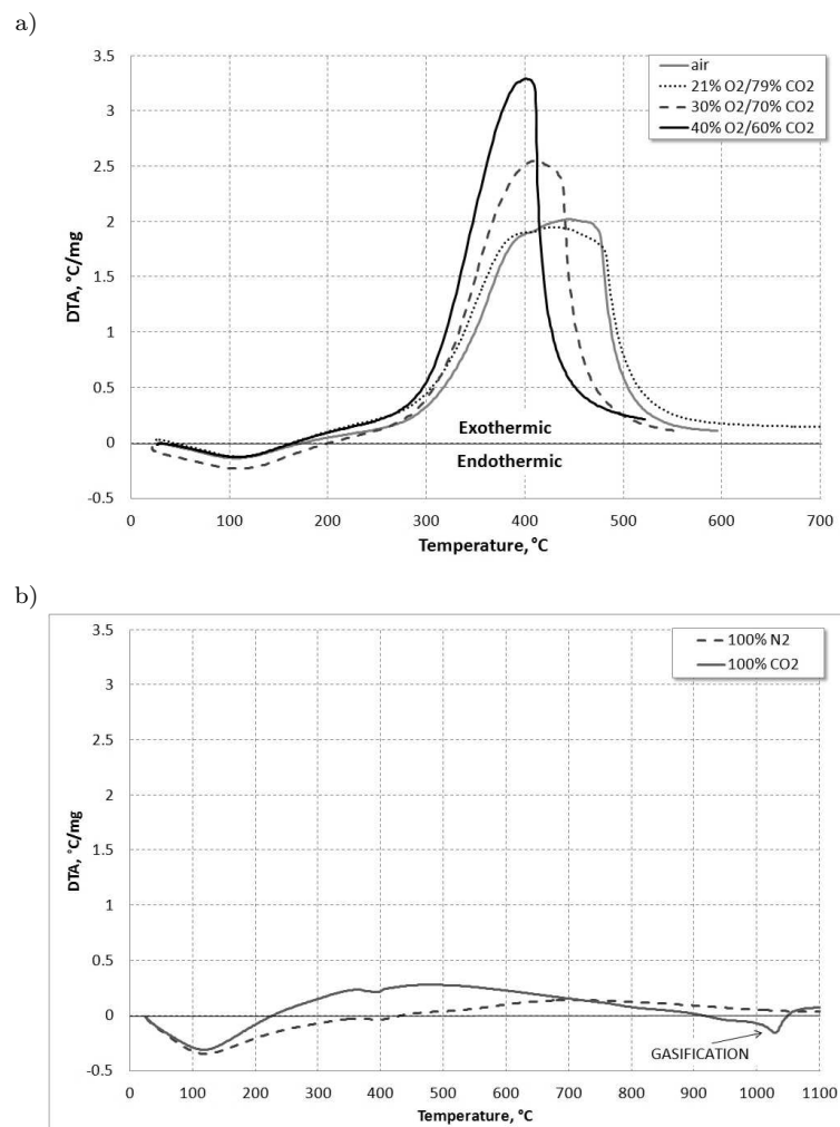
Figure 7: DTA curves of wooden biomass during combustion (a) and pyrolysis (b).
