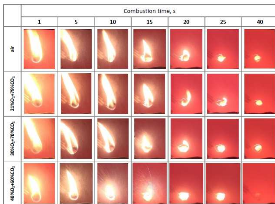
Figure 2: Combustion of biomass particles in air and O 2 /CO 2 mixtures at 850 °C.
