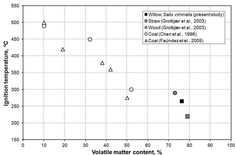
Figure 6: Relationship between fuel volatile matter content (dry basis) and TG ignition temperature for various solid fuels.
