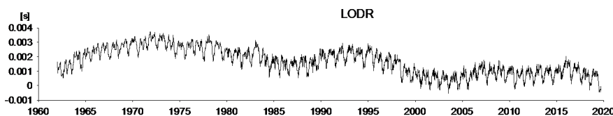
Figure 1. LODR daily time series data
