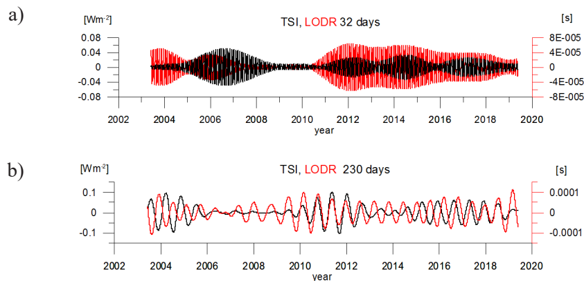
Figure 5. Oscillations in TSI (black) and LODR (red) time series with central periods of a) 32 days and b) 230 days computed by the FTBPF ( \lambda=0.001 )
